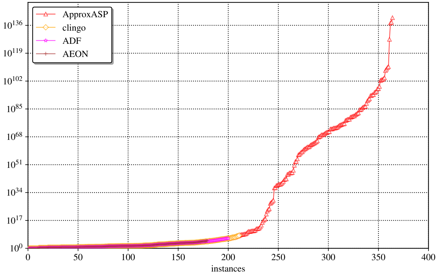
number of Minimal Trap Spaces
