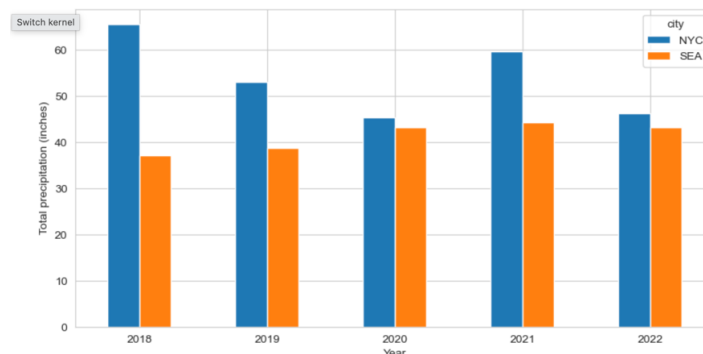
Figure 1. Total precipitation per year
