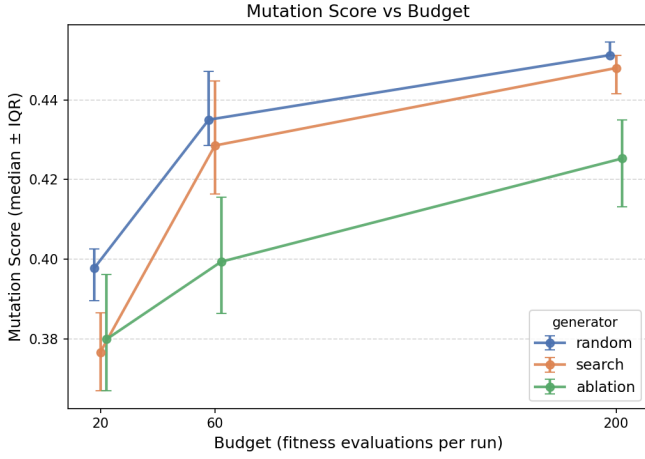
Fig. 1. Mutation score (median \pm IQR) versus budget. The guided search tracks but does not exceed random; it separates clearly from the unguided ablation as the budget grows.
