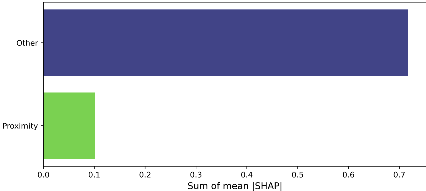
Model 1 (RF) SHAP importance by theme
