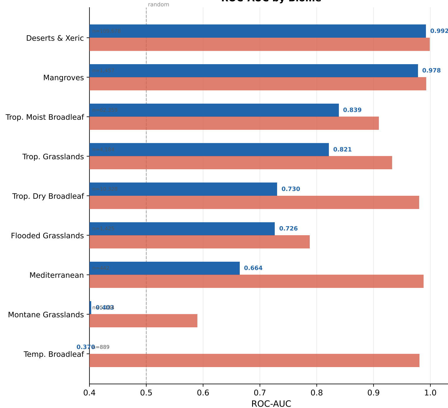
ROC-AUC by Biome
