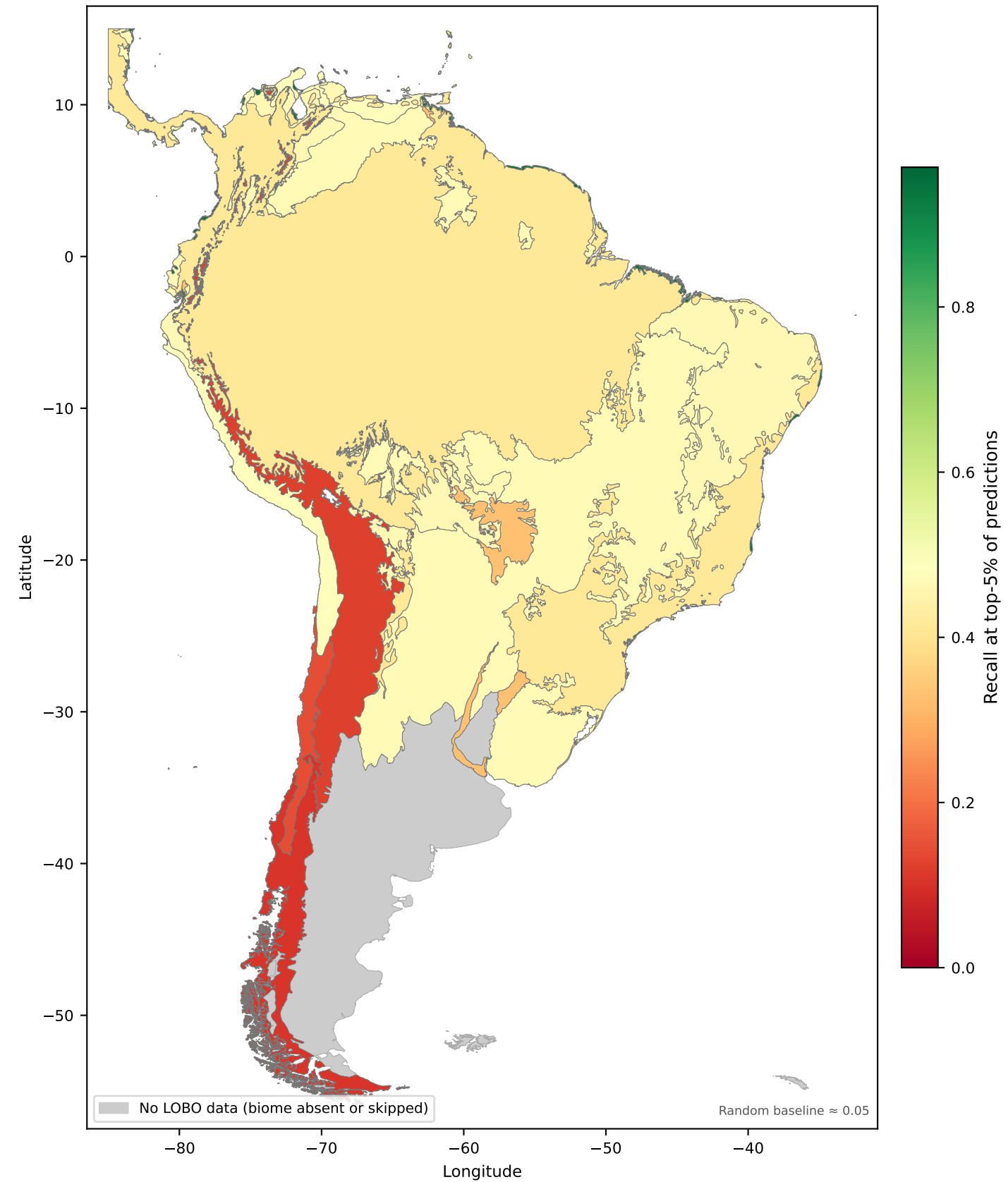
LOBO Recall@top-5% (fraction of PA events captured)
