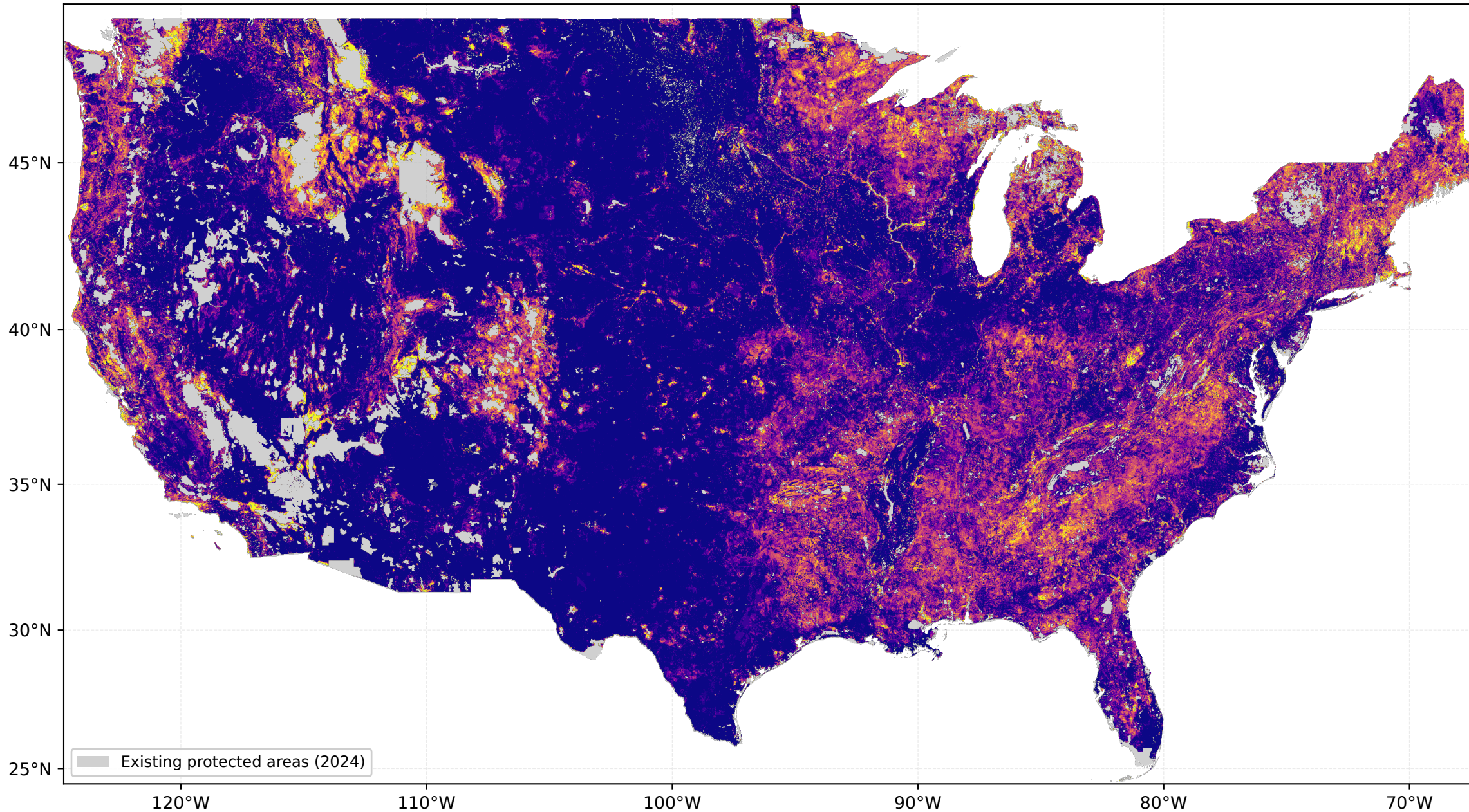
BAU Forecast: P(Protected-Area Designation by 2030) — USA Deployment model (2001-2019), unprotected pixels as of 2024
