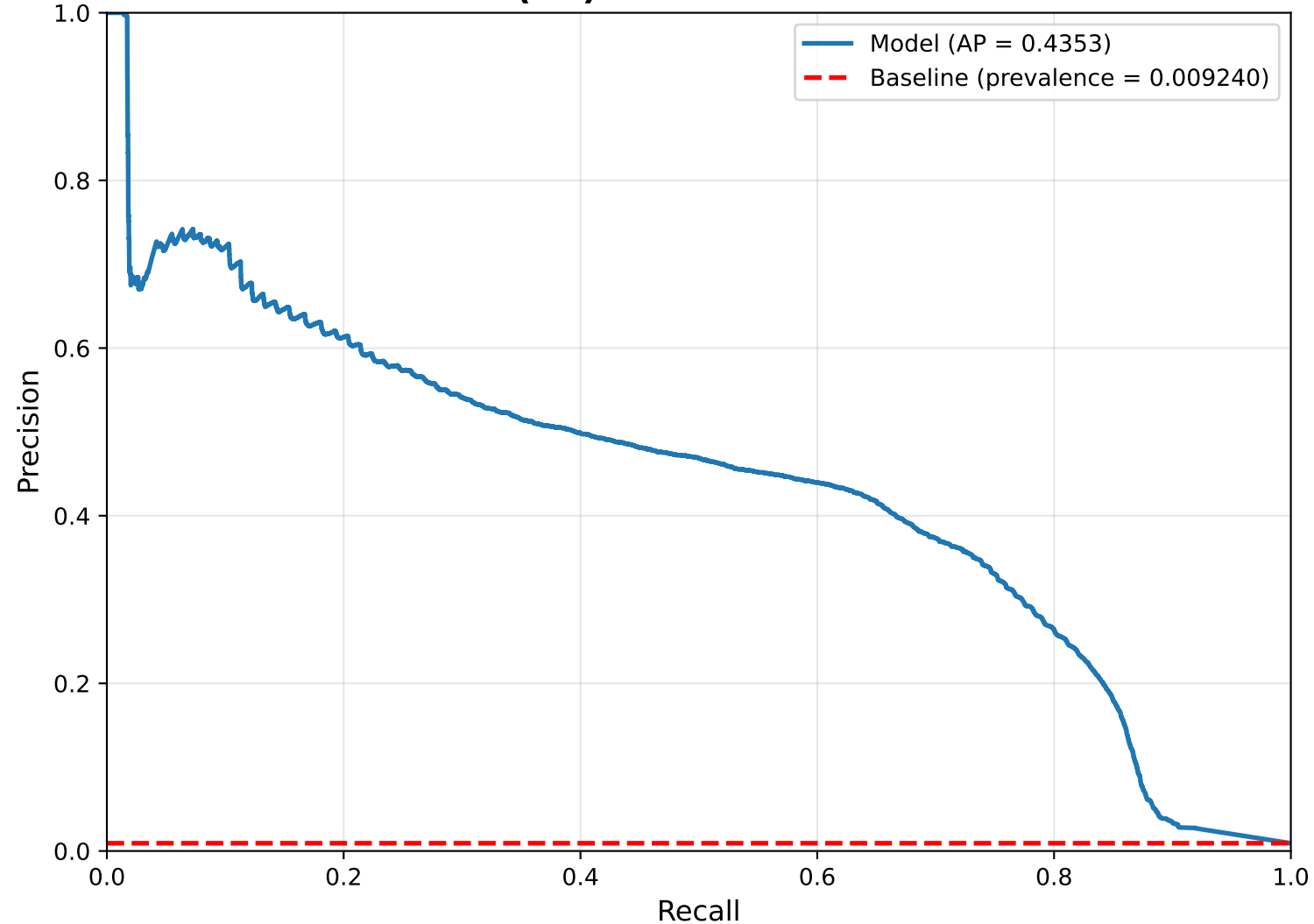
Model C (RF) Precision-Recall Curve
