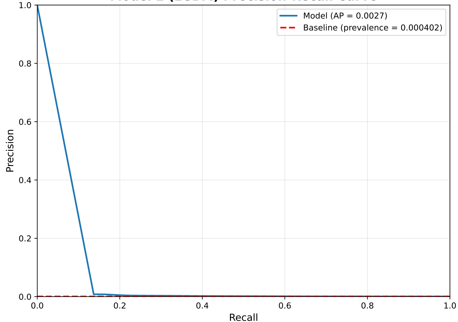
Model 2 (LGBM) Precision-Recall Curve
