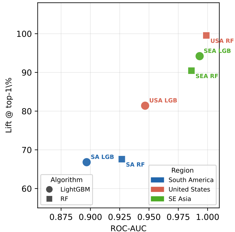
(b) Discrimination vs. Targeting Effectiveness
