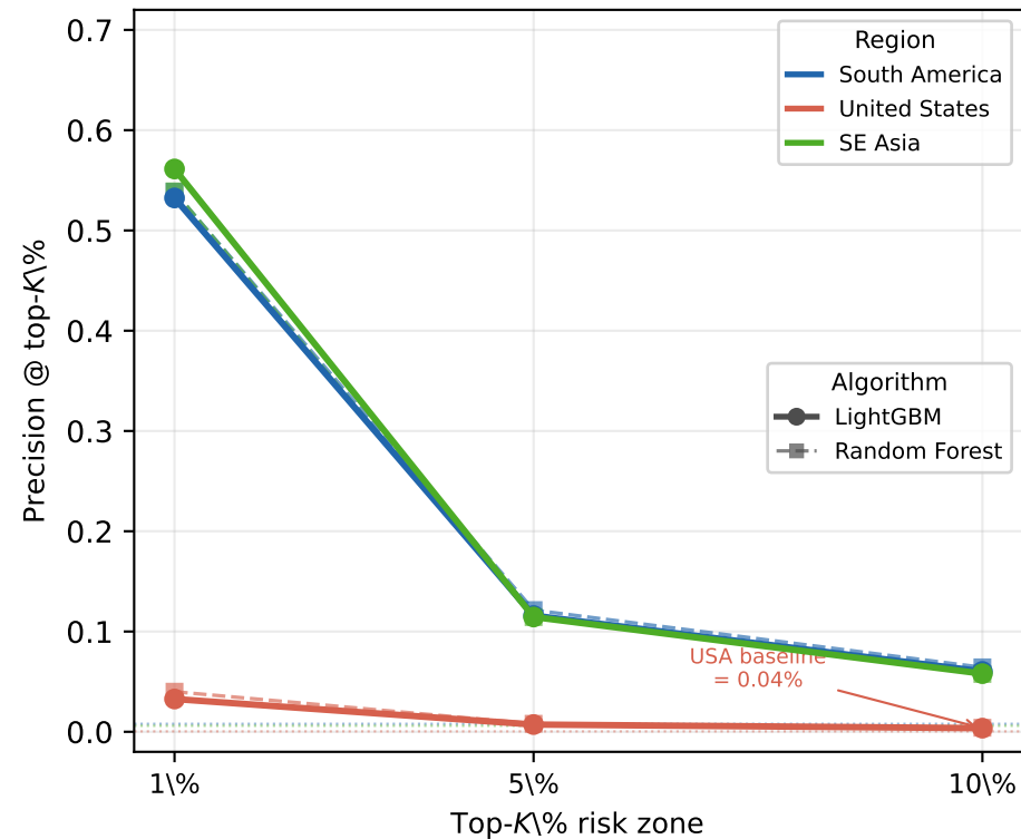
(a) Targeting Precision at Different Risk Thresholds
