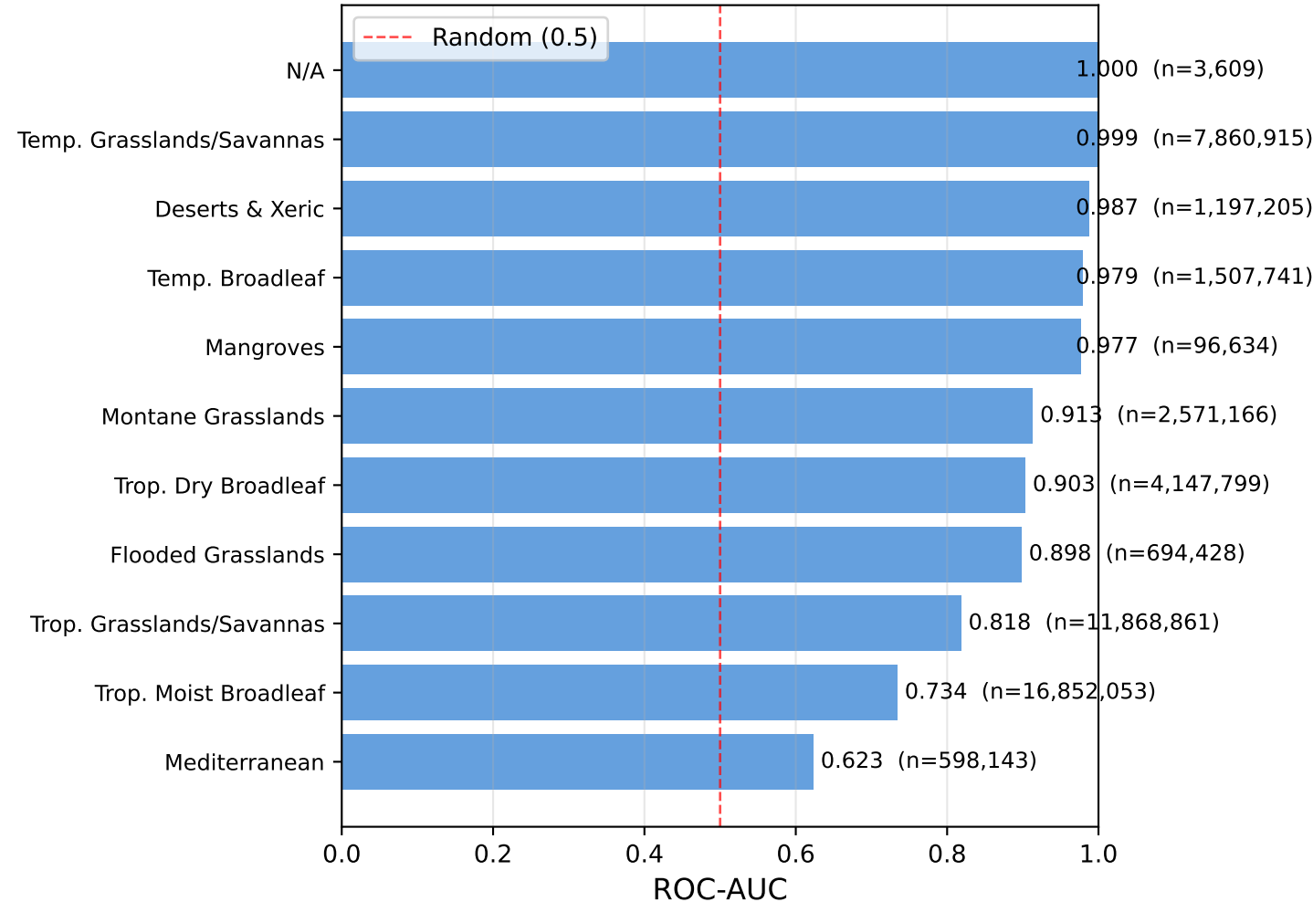
ROC-AUC by Biome
