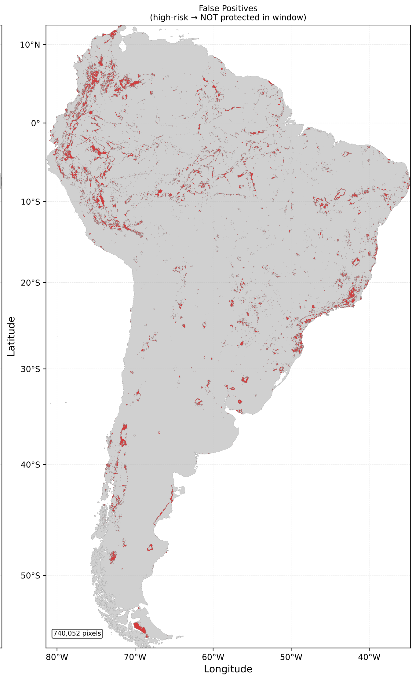
False Positive Analysis — T=2015 Backtest (South America) Top-5% risk zone: 52,662 true positives (green) / 740,052 false positives (red) precision=0.066
