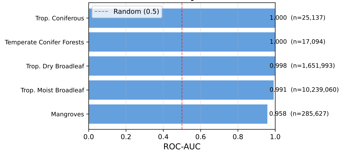
ROC-AUC by Biome
