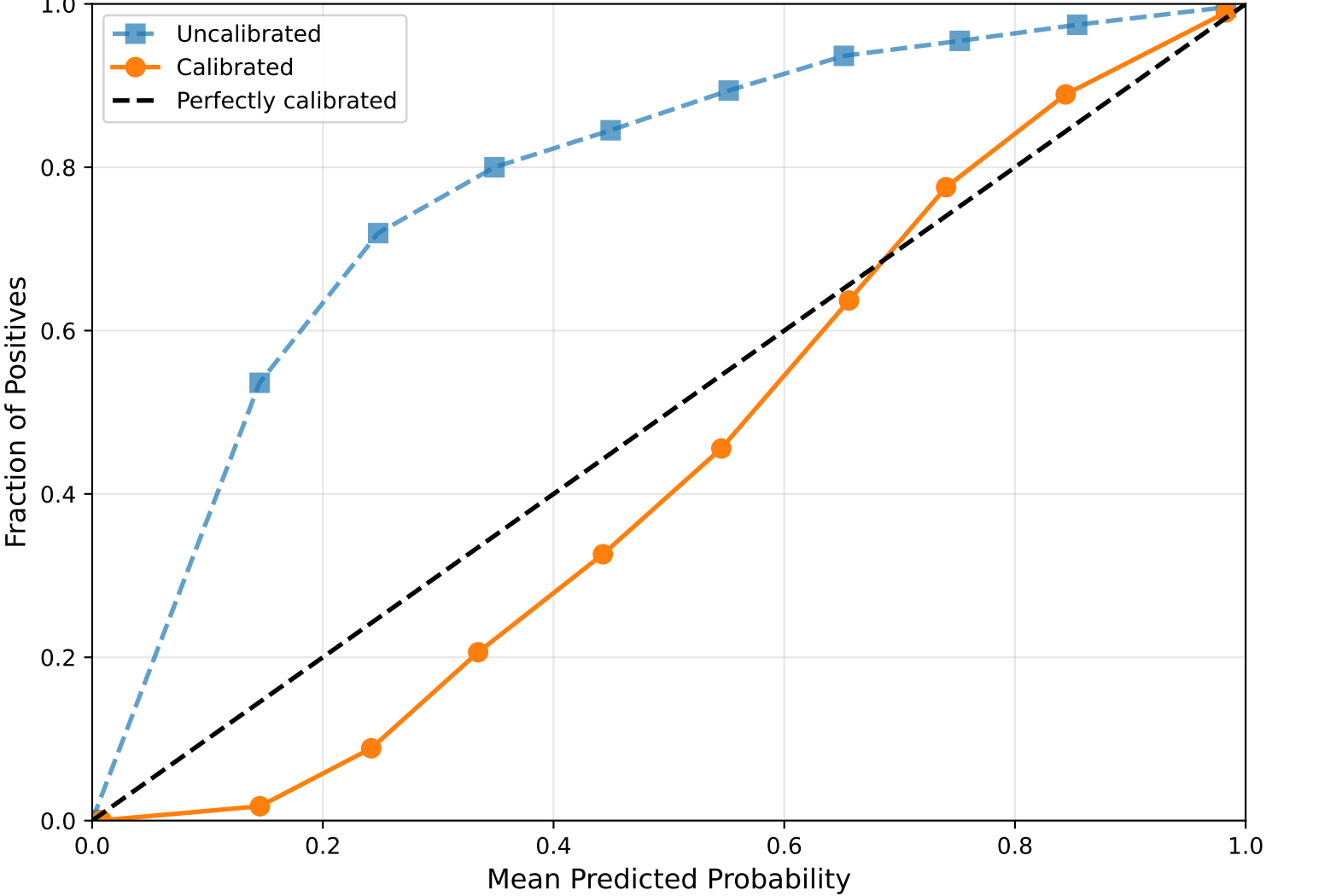
Model 3 (LGBM) Calibration Reliability Diagram (Uniform Bins, n=10)
