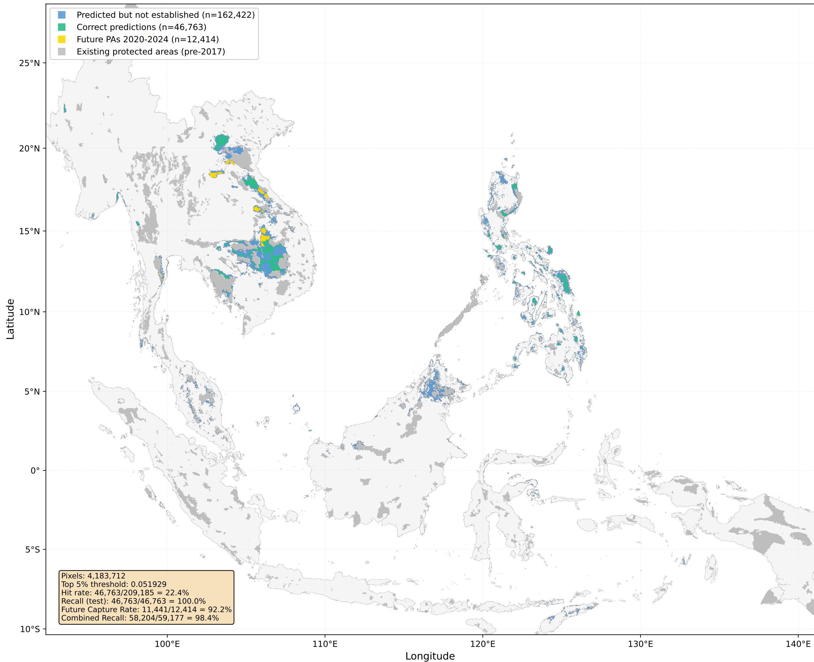
Model 3 (RF): Predicted Risk vs Actual Establishments (2017-2019)
