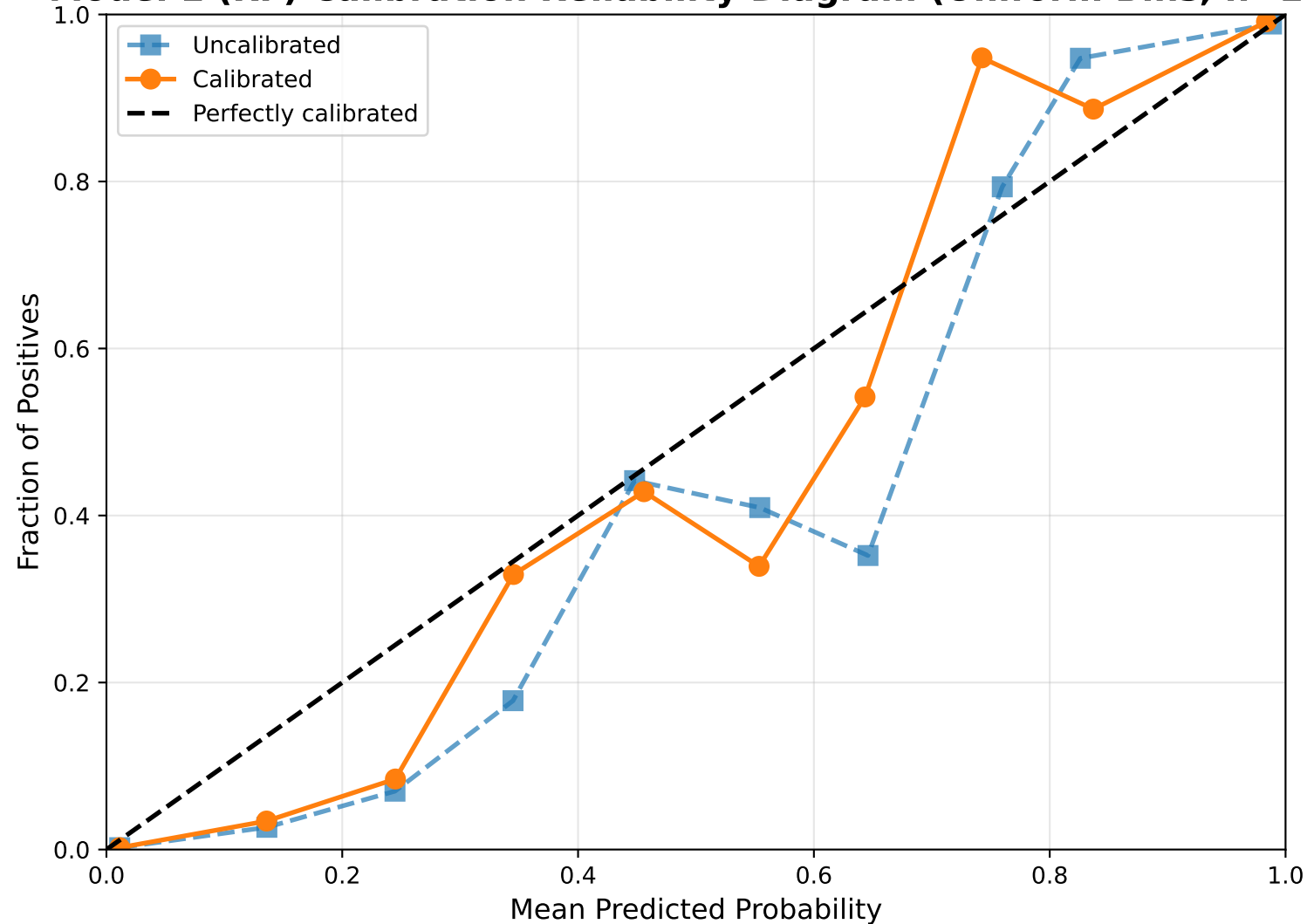
Model 1 (RF) Calibration Reliability Diagram (Uniform Bins, n=10)
