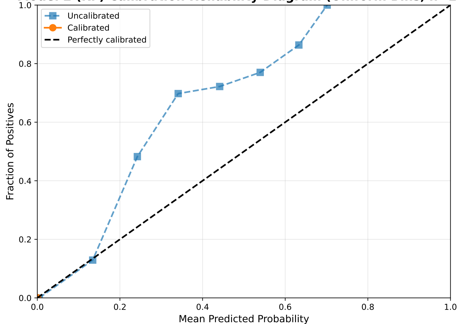
Model 2 (RF) Calibration Reliability Diagram (Uniform Bins, n=10)
