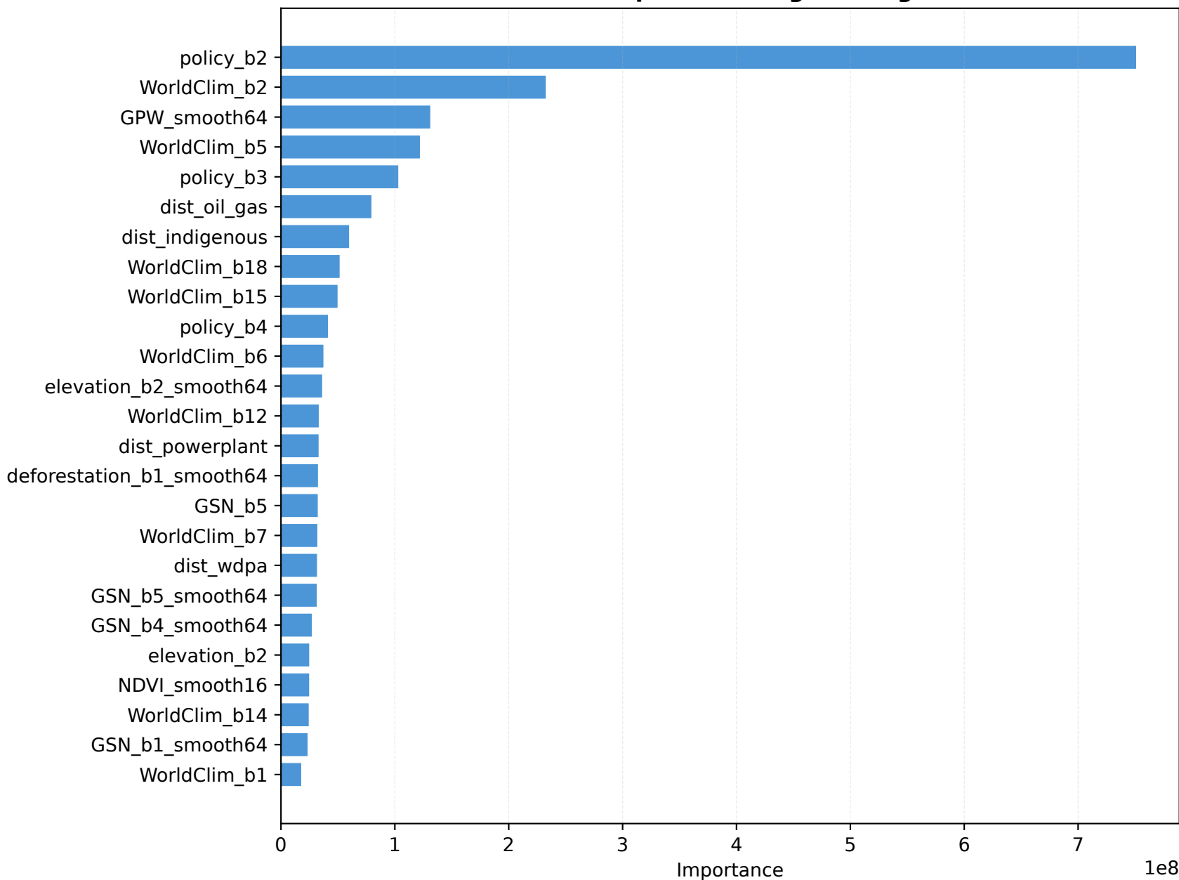
Feature Importance (LightGBM gain)
