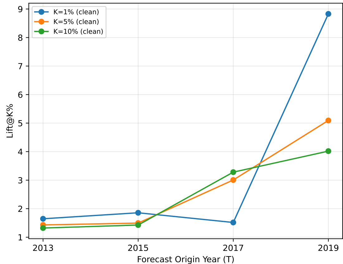
Pseudo-forecast Backtesting (LGBM): Precision@K% and Lift@K%
