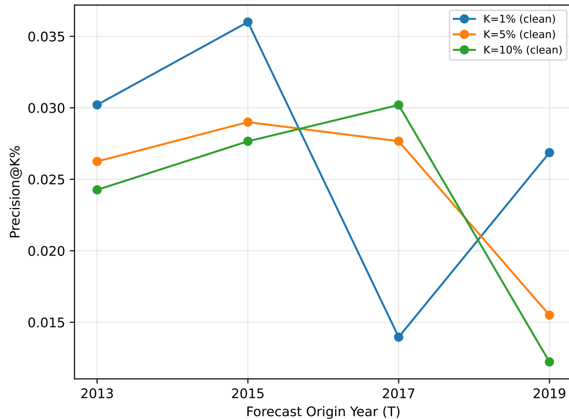
Pseudo-forecast Backtesting (LGBM): Precision@K% and Lift@K%
