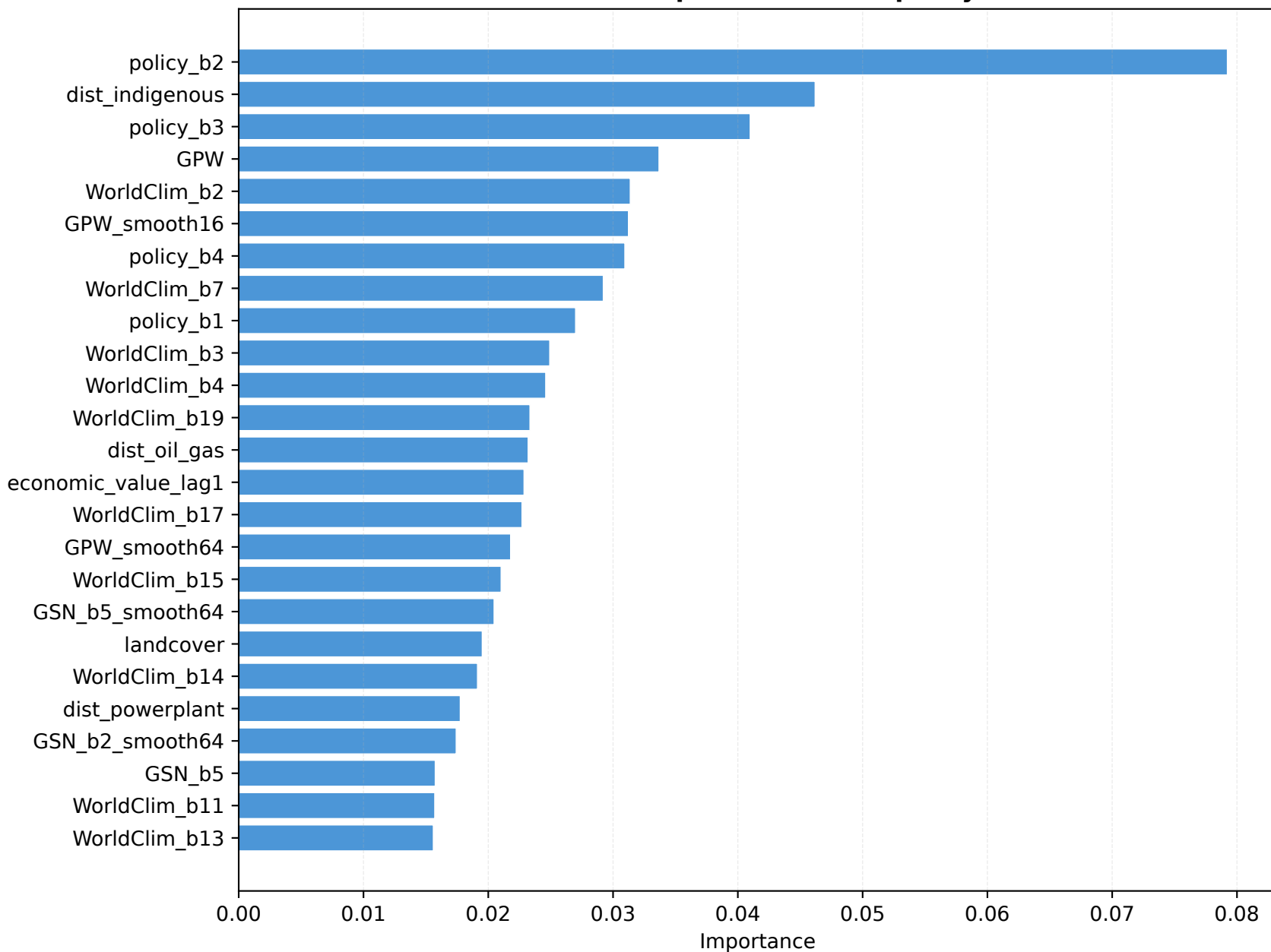
Feature Importance (RF impurity)
