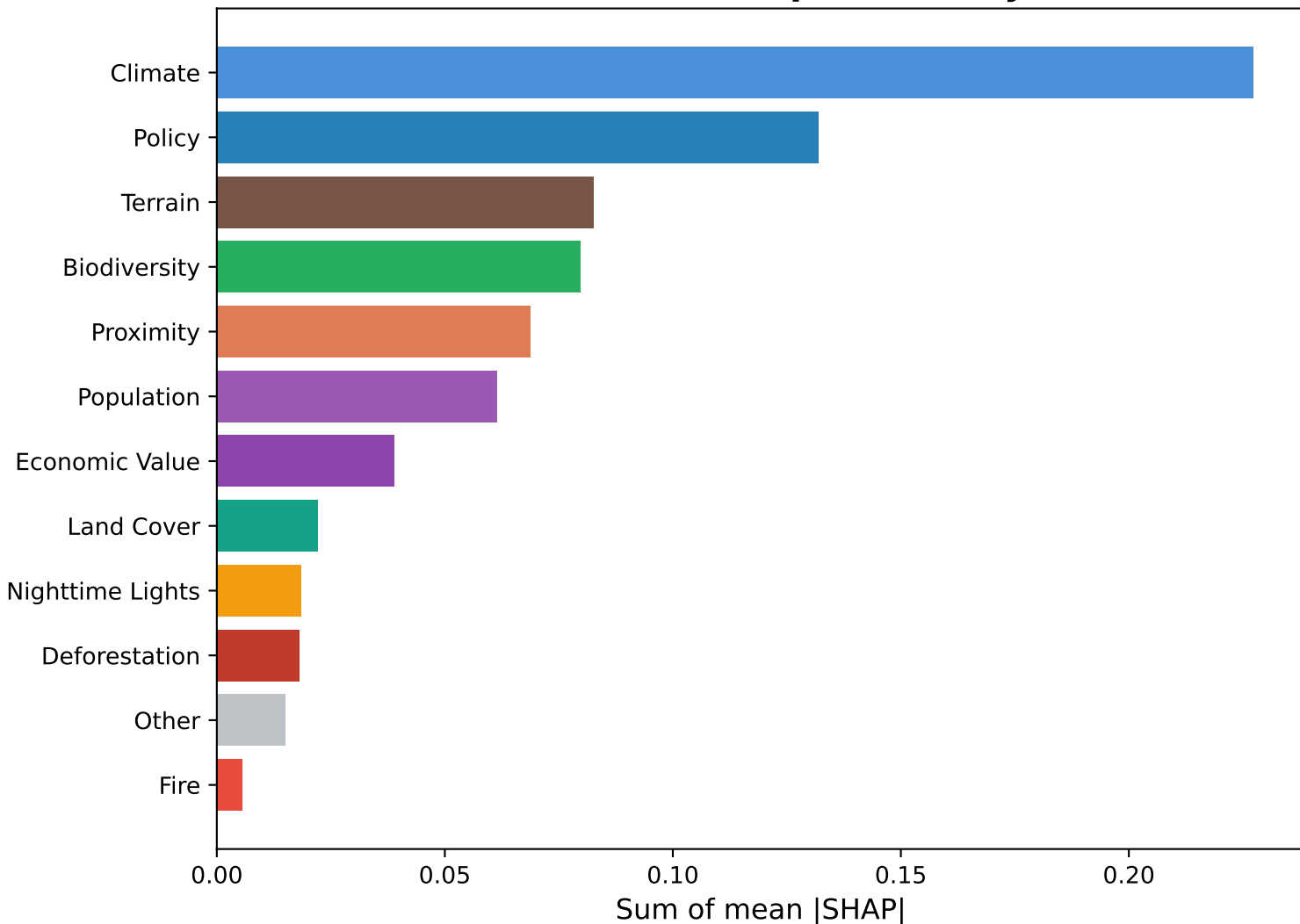
Model 3 (RF) SHAP importance by theme
