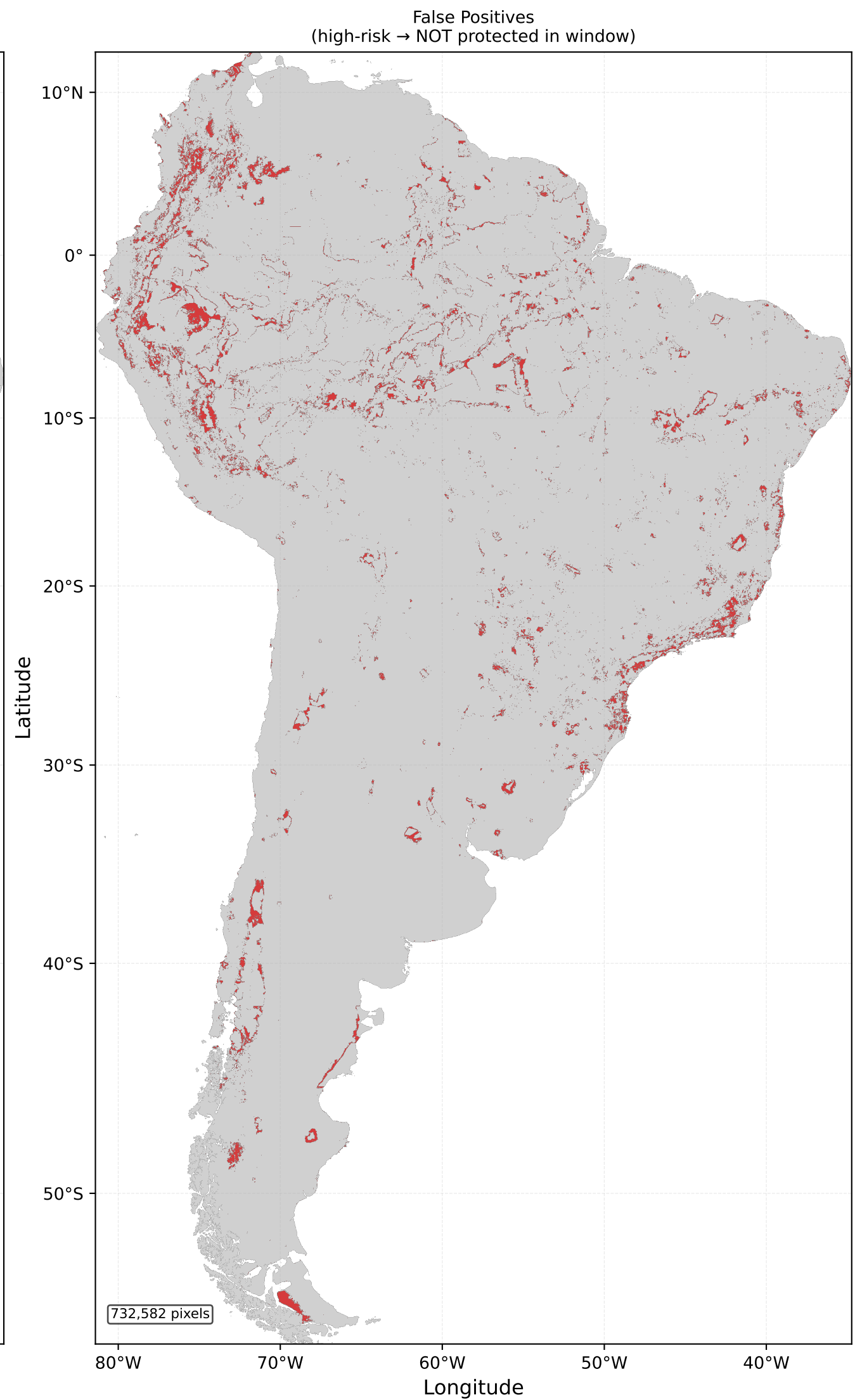
False Positive Analysis — T=2015 Backtest (South America) Top-5% risk zone: 60,132 true positives (green) / 732,582 false positives (red) precision=0.076
