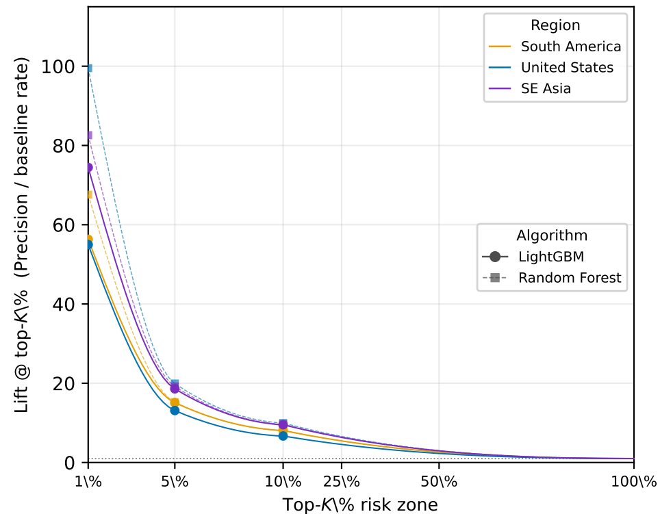
(a) Targeting Lift at Different Risk Thresholds
