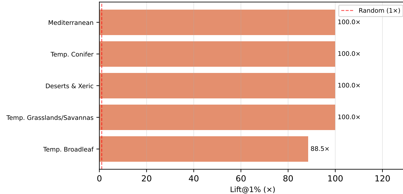
Lift@1% by Biome
