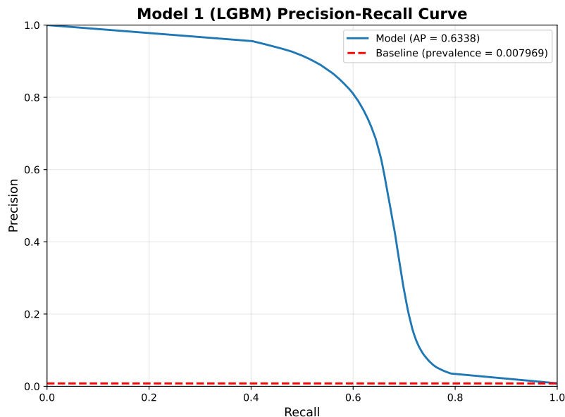
Figure 2: Precision–Recall curve for the South America LightGBM model on the temporal test set (2017–2019). The dashed horizontal line shows the random-classifier baseline (equal to the positive rate, \approx 0.8\% ). The large area between the PR curve and the baseline quantifies the model’s discrimination advantage over random selection.
