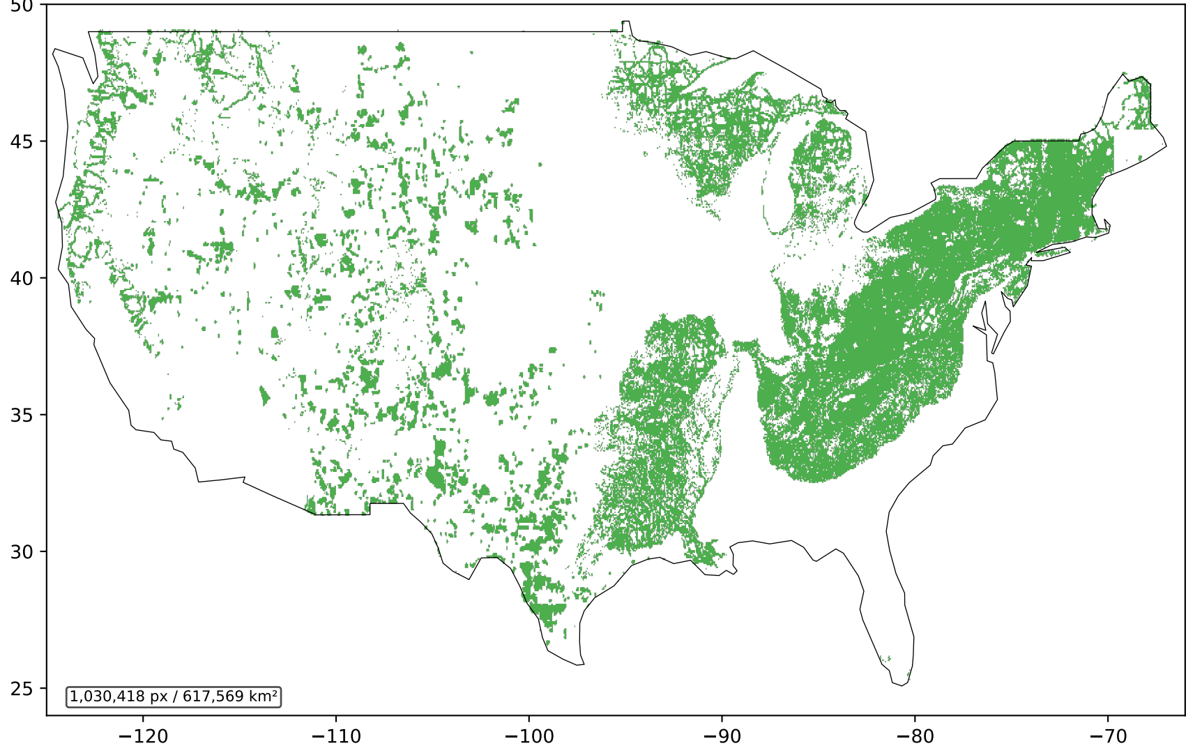
Biodiversity Priority (GSN_b1==1) High-priority unprotected pixels
