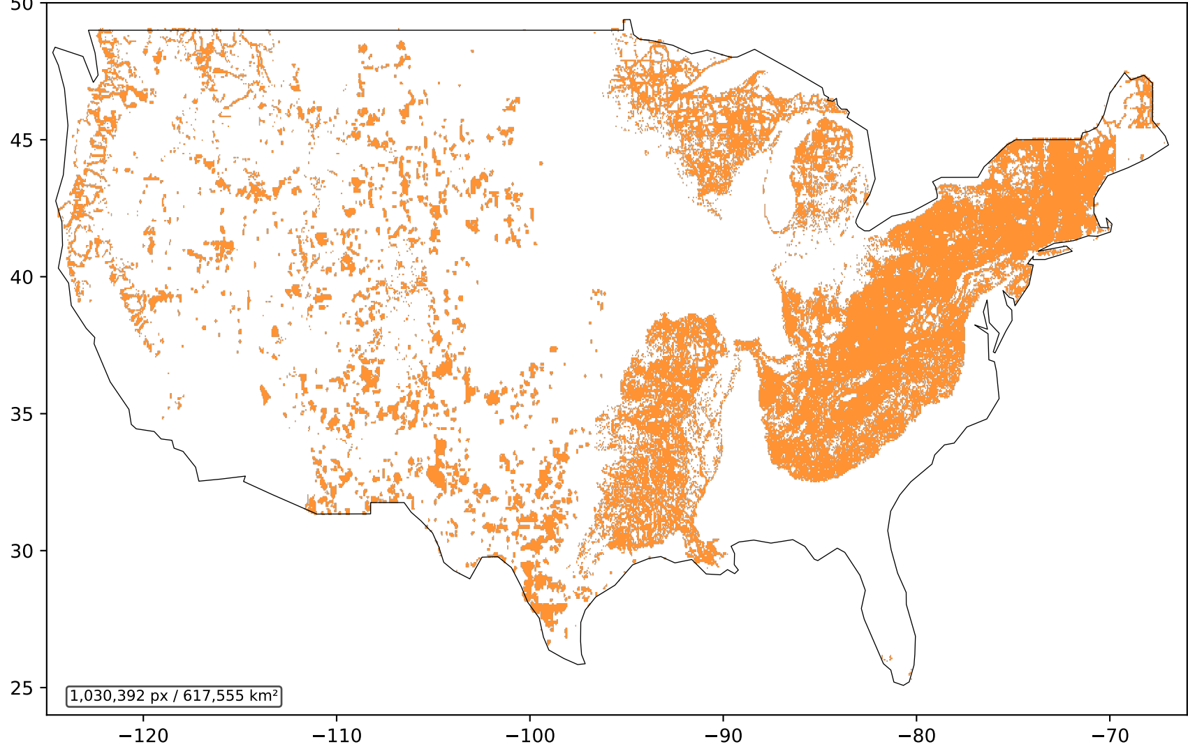
Gap: Biodiversity Priority not in BAU (high-value land left unprotected)
