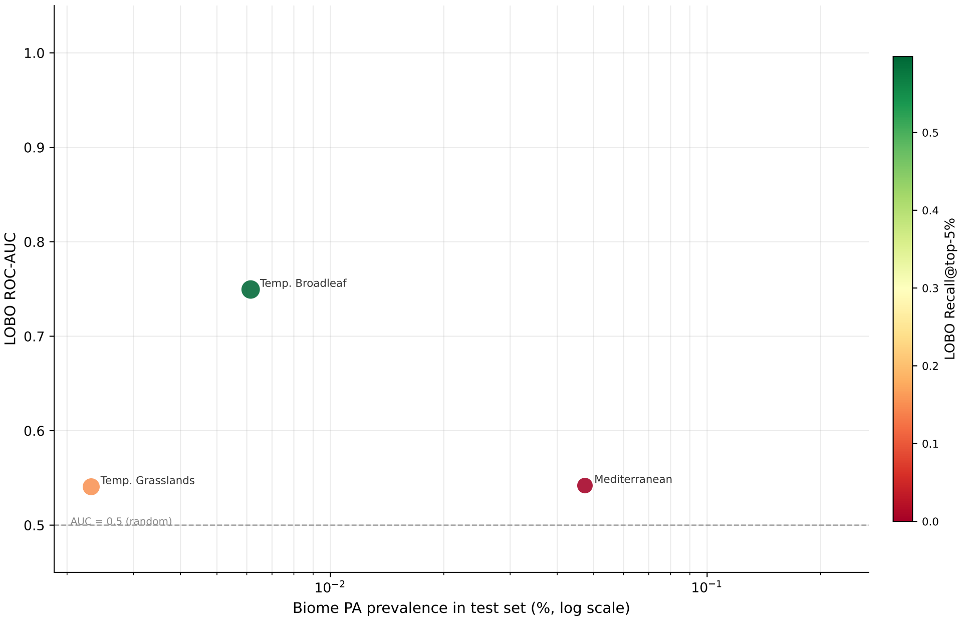
LOBO Generalisation vs. Biome PA Prevalence Bubble size \propto \sqrt{(\text{PA events in held-out test set})}
