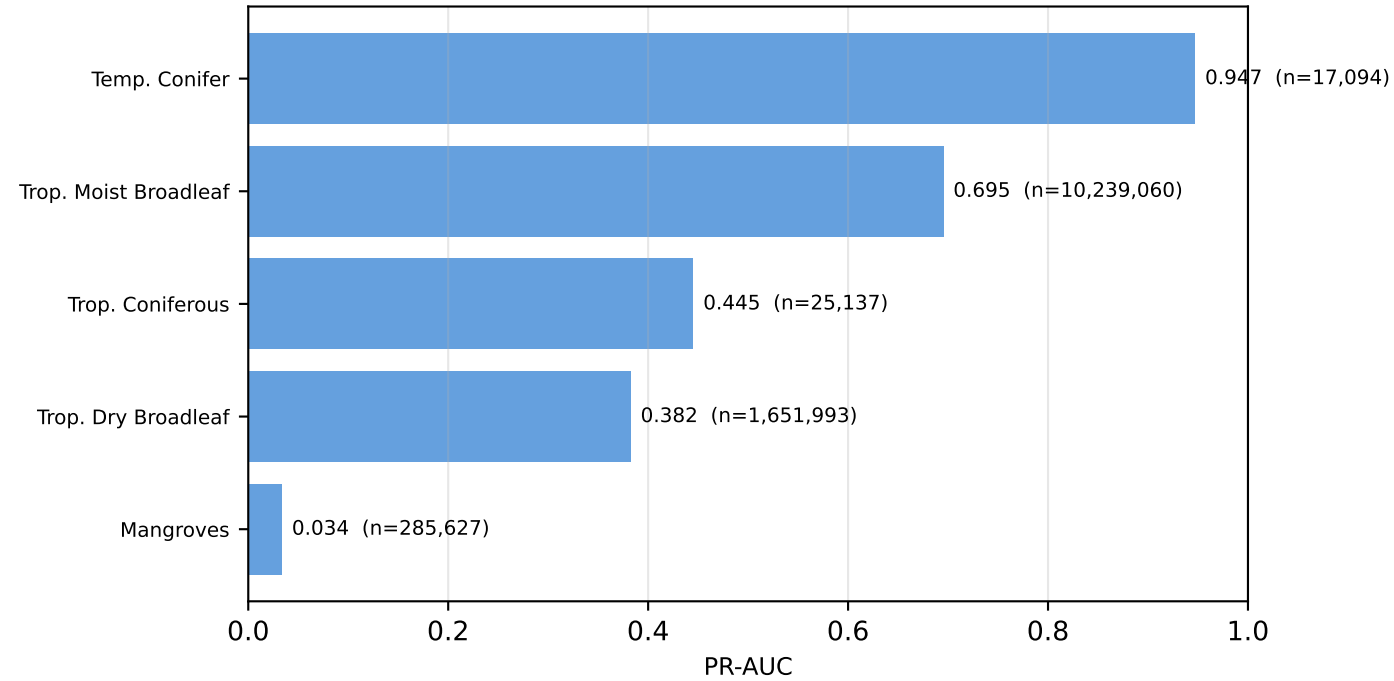
PR-AUC by Biome
