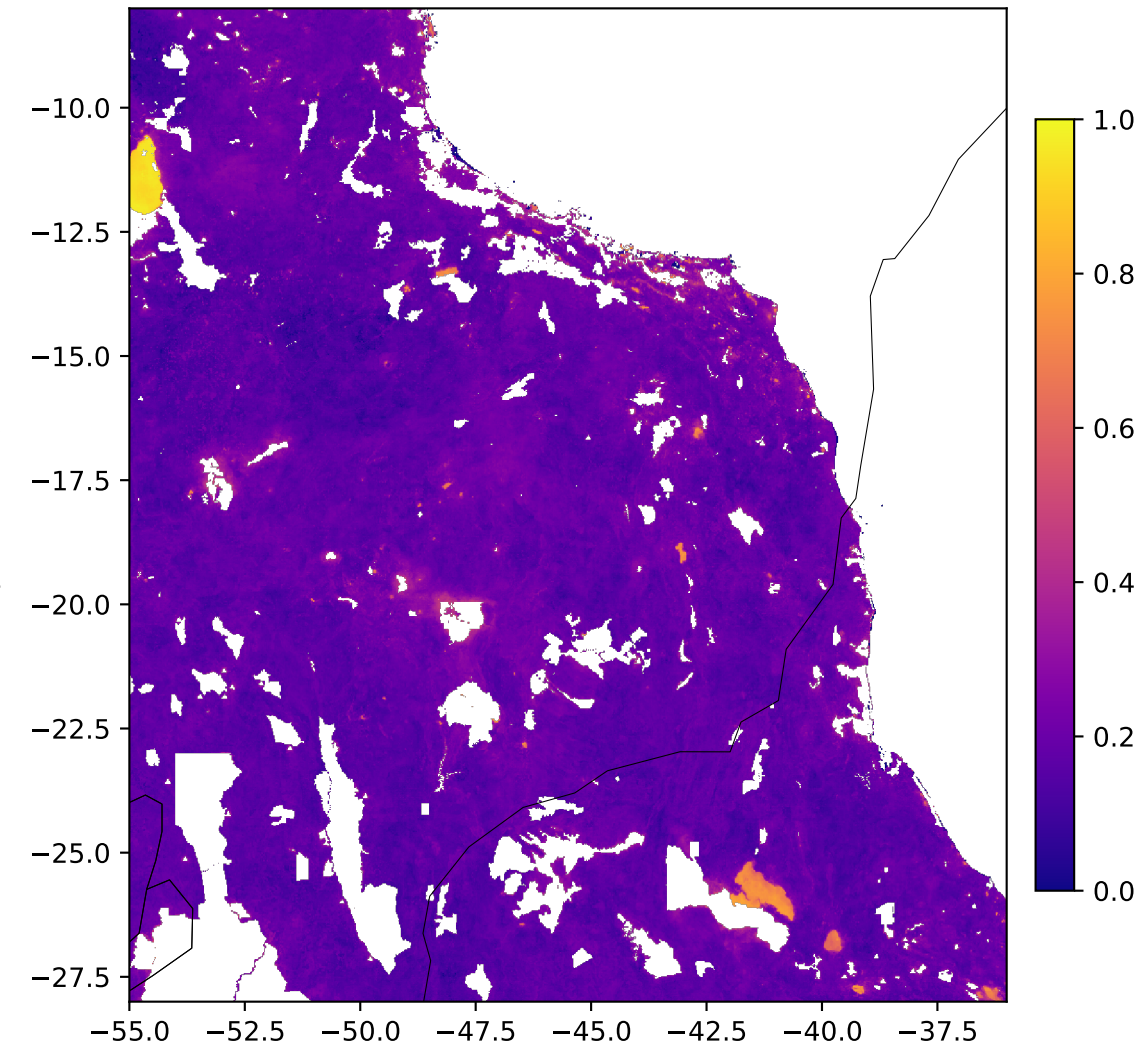
Hotspot Zoom-ins — South America (RF) Top row: P(protection) probability | Bottom row: top-1% risk zone Cerrado / Atlantic Forest
