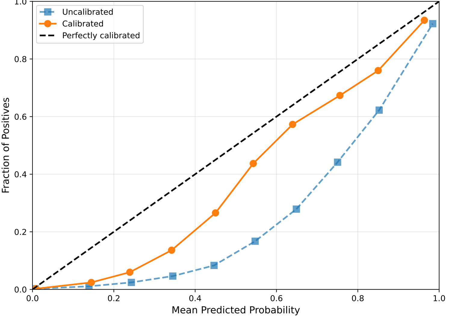
Model 1 (LGBM) Calibration Reliability Diagram (Uniform Bins, n=10)
