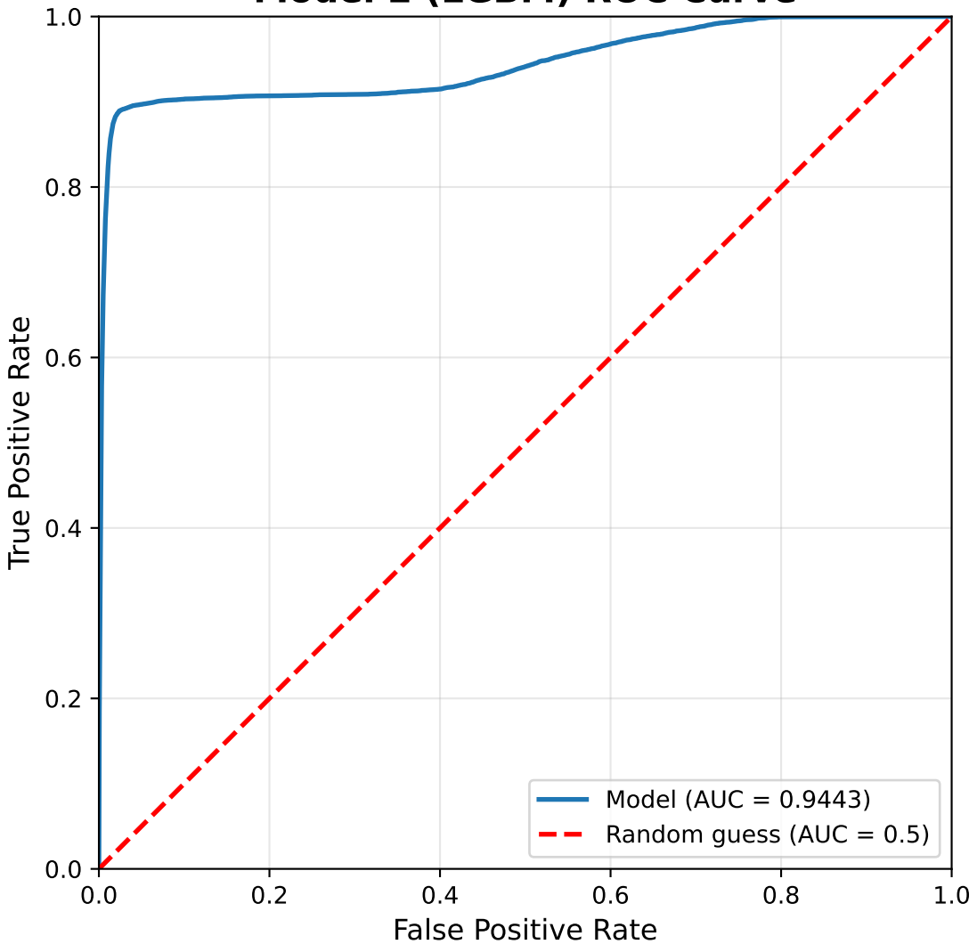
Model 2 (LGBM) ROC Curve
