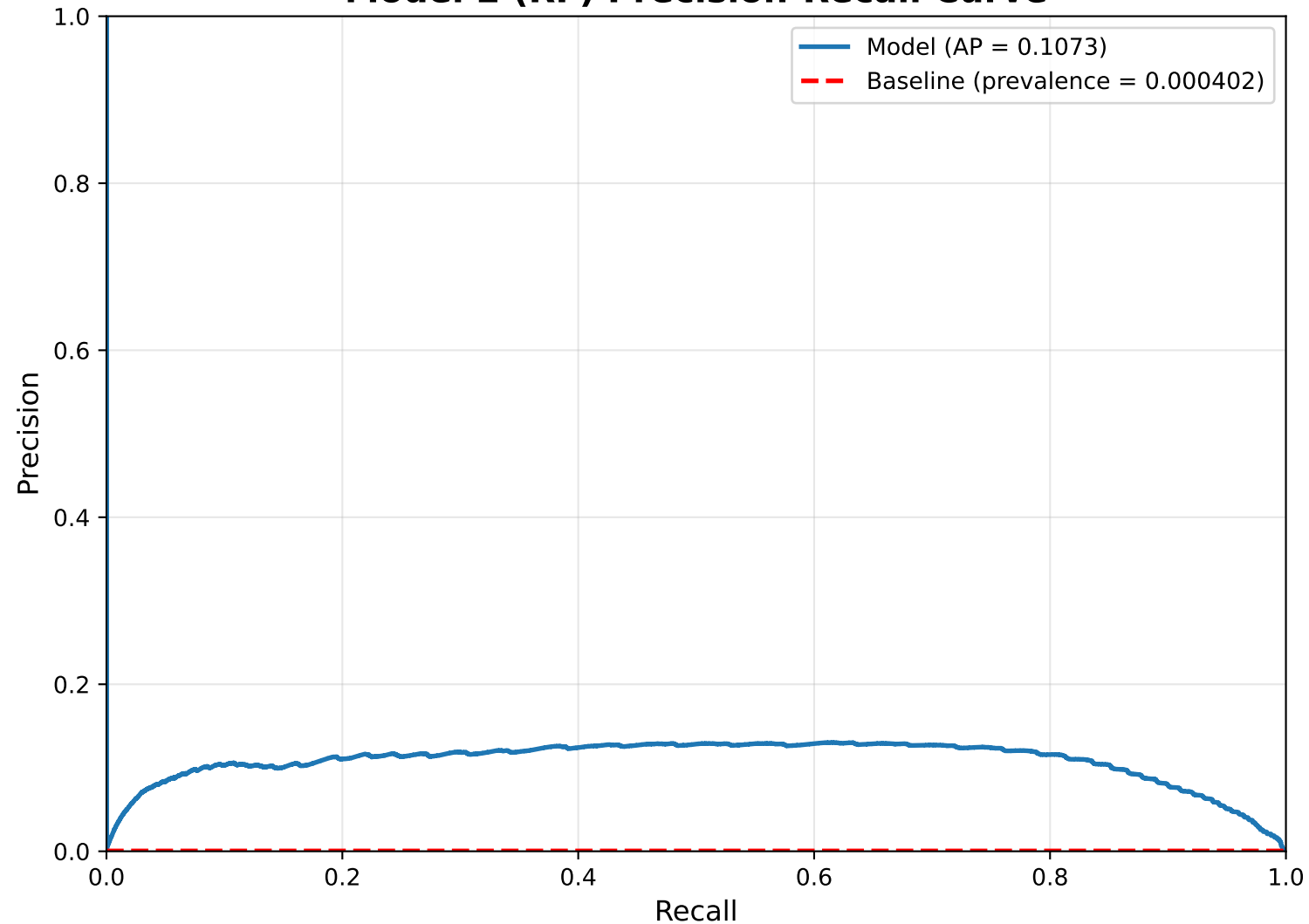
Model 2 (RF) Precision-Recall Curve
