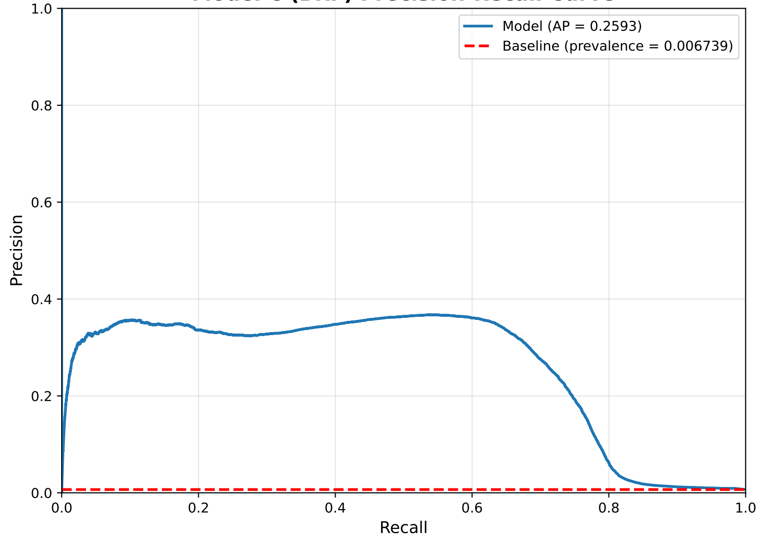
Model C (BRF) Precision-Recall Curve
