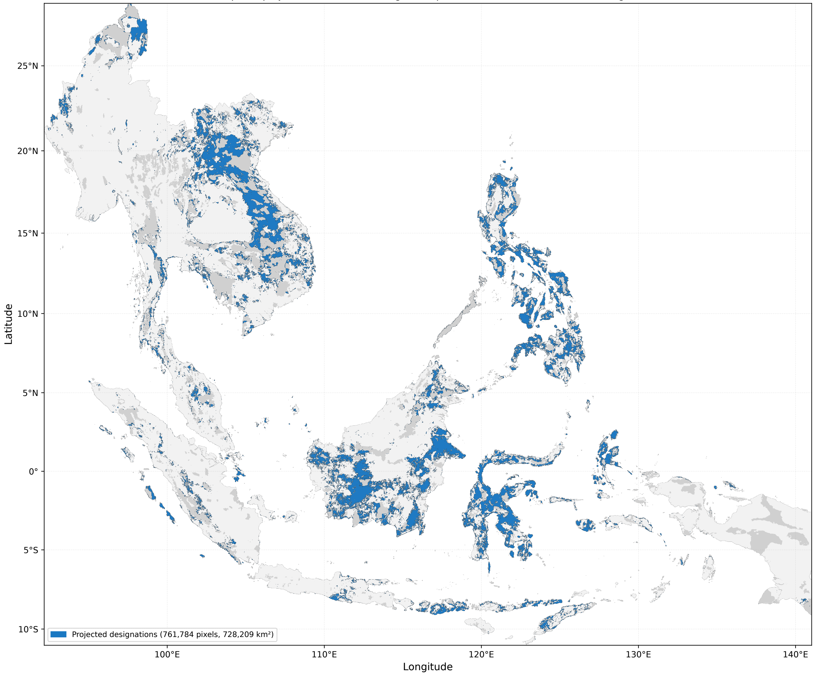
30x30 Full Scenario (→30% South East Asia coverage) Spatial projection if historical designation preferences continue to 30% coverage
