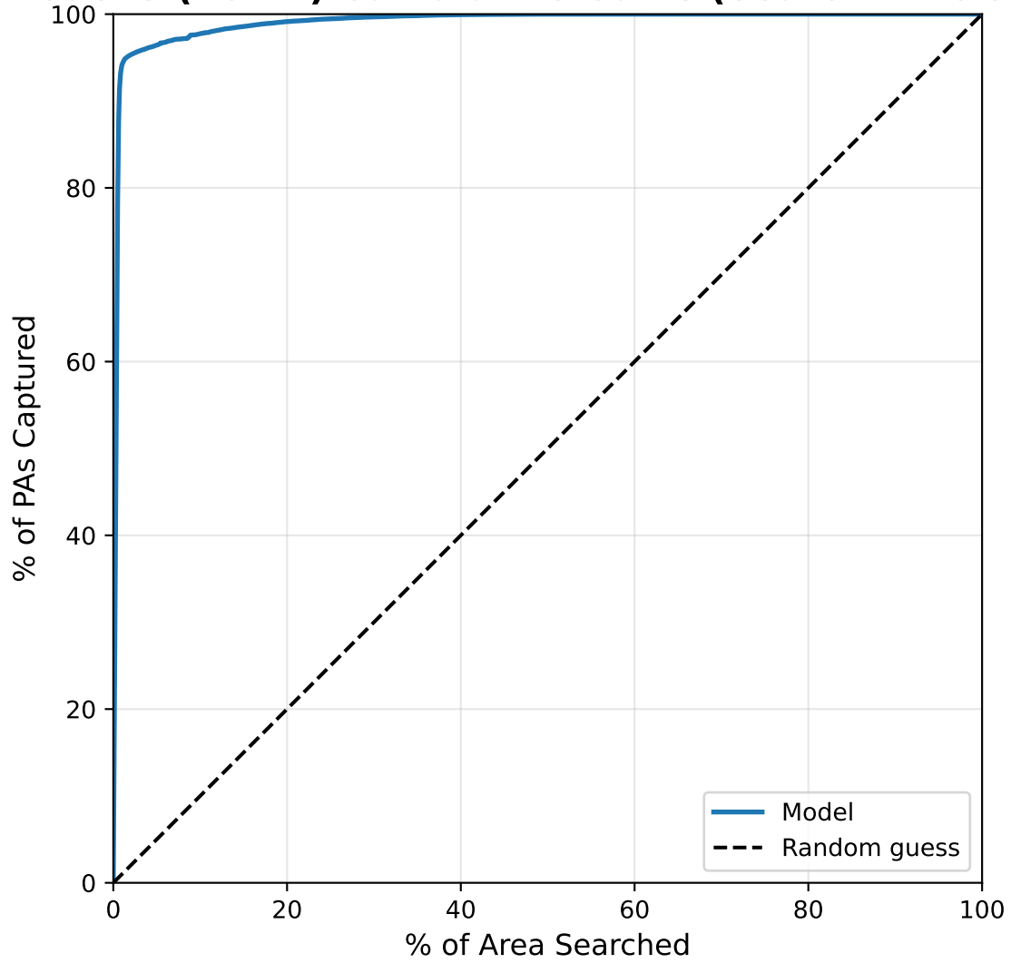
Model 3 (LGBM) Cumulative Gains (Search Efficiency)
