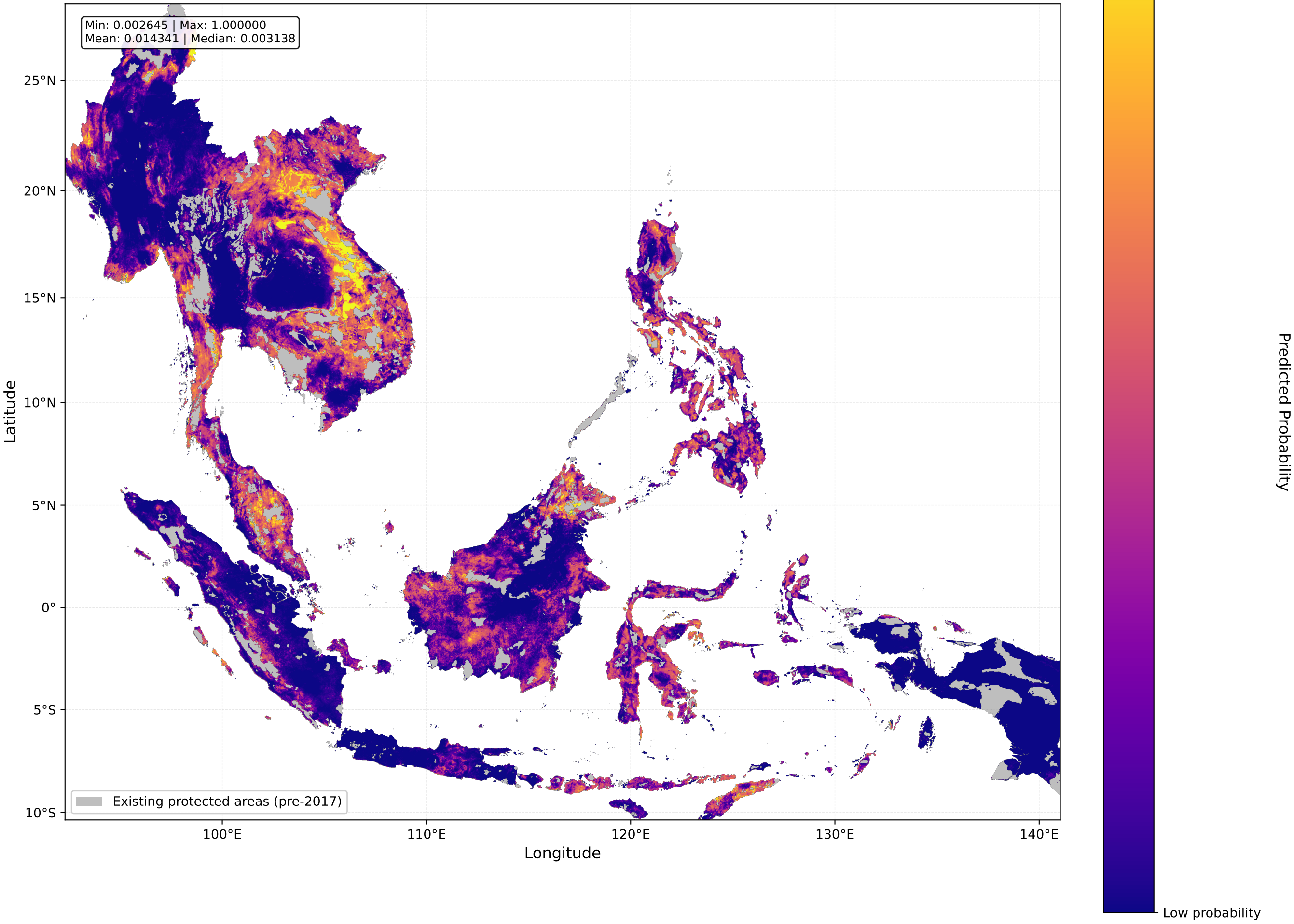
Model 3 (LGBM) Probability Map (Calibrated Probabilities)
