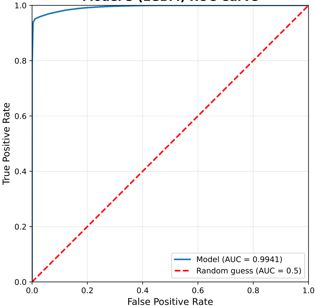
Model 3 (LGBM) ROC Curve
