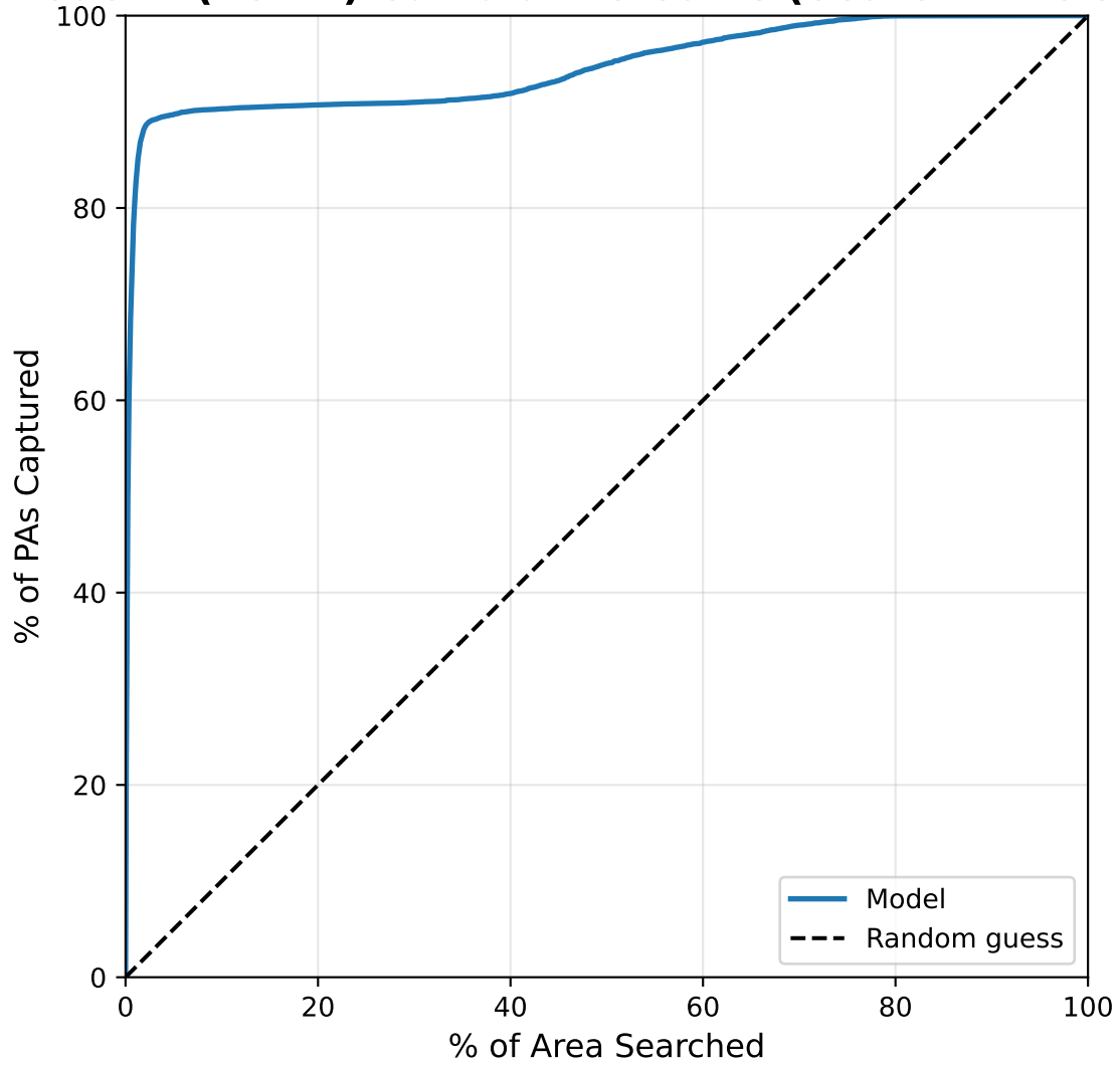
Model 2 (LGBM) Cumulative Gains (Search Efficiency)
