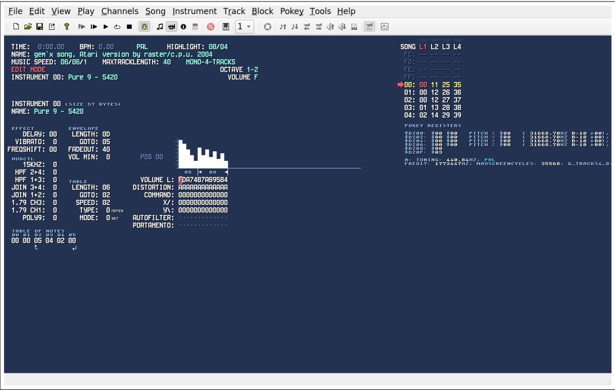
Figure 4.2. The instrument part (INSTRUMENT EDIT) with an instrument loaded.
