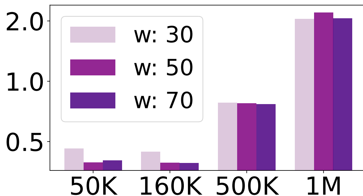
Relation: equal
