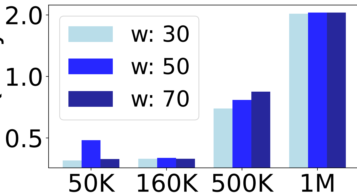
Relation: meets
