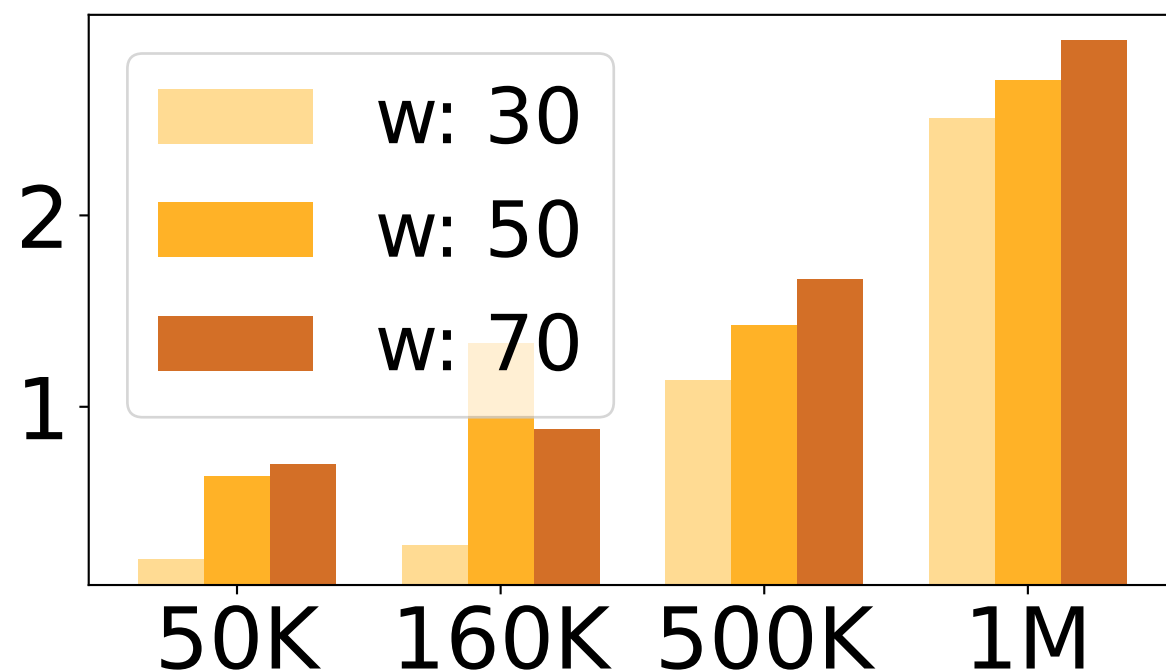
Relation: meets
