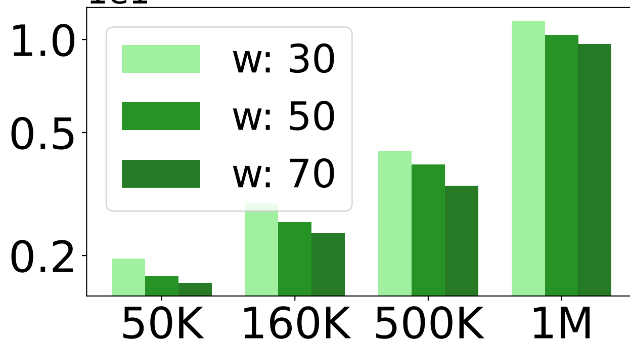
Relation: before
