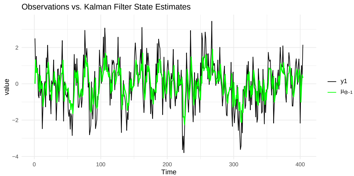
Figure 3: Kalman Filter state estimates for y_1
