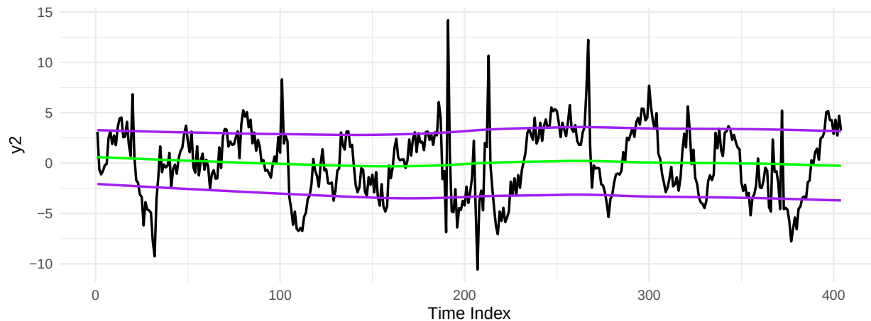
Figure 4: Time series y_2 with robust loess smooth for mean and standard deviation.
