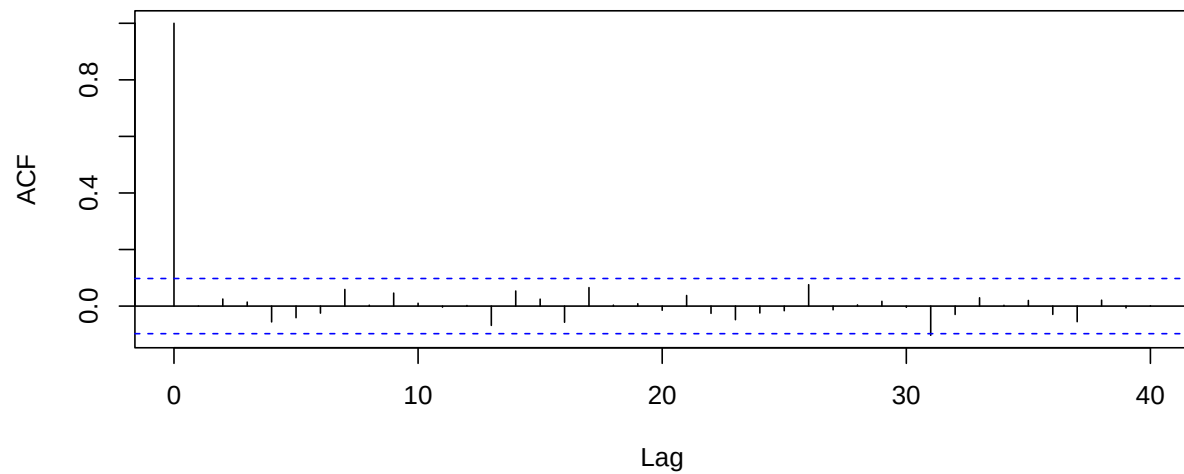
Figure 10: ACF for standardized innovations for y_1
