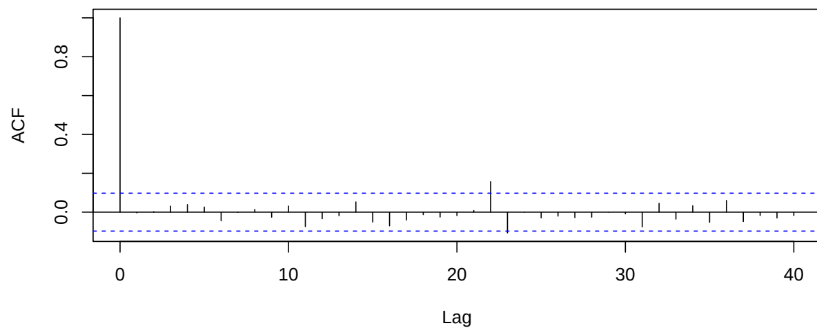
Figure 11: ACF for standardized innovations for y_1
