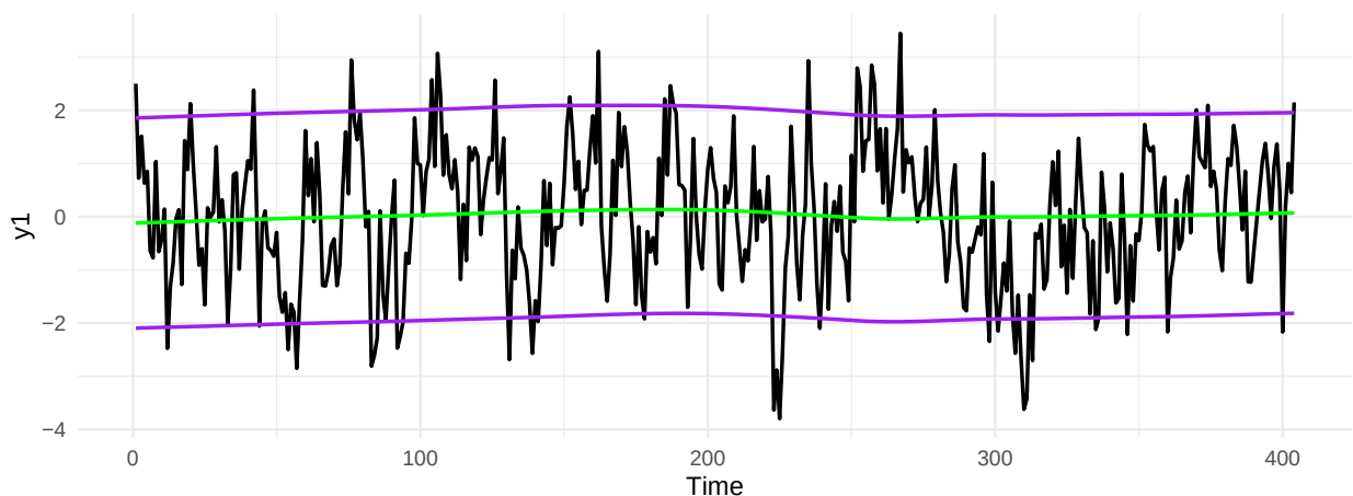
Figure 2: Time series y_1 with robust loess smooth for mean and standard deviation.
