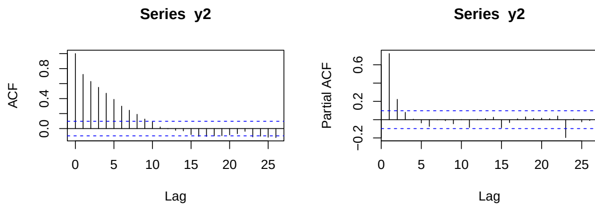
Figure 5: ACF and PACF for y_2
