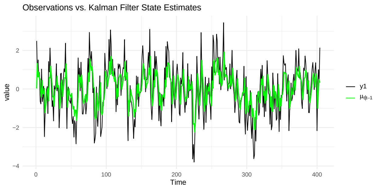
Figure 7: Kalman Filter state estimates for y_1
