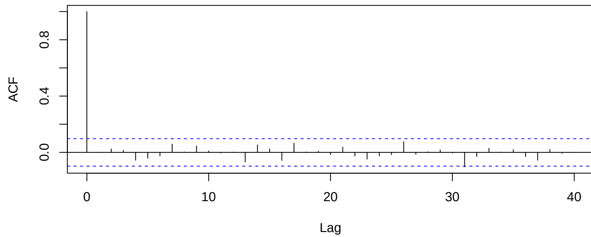
Figure 6: ACF for standardized innovations for y_1
