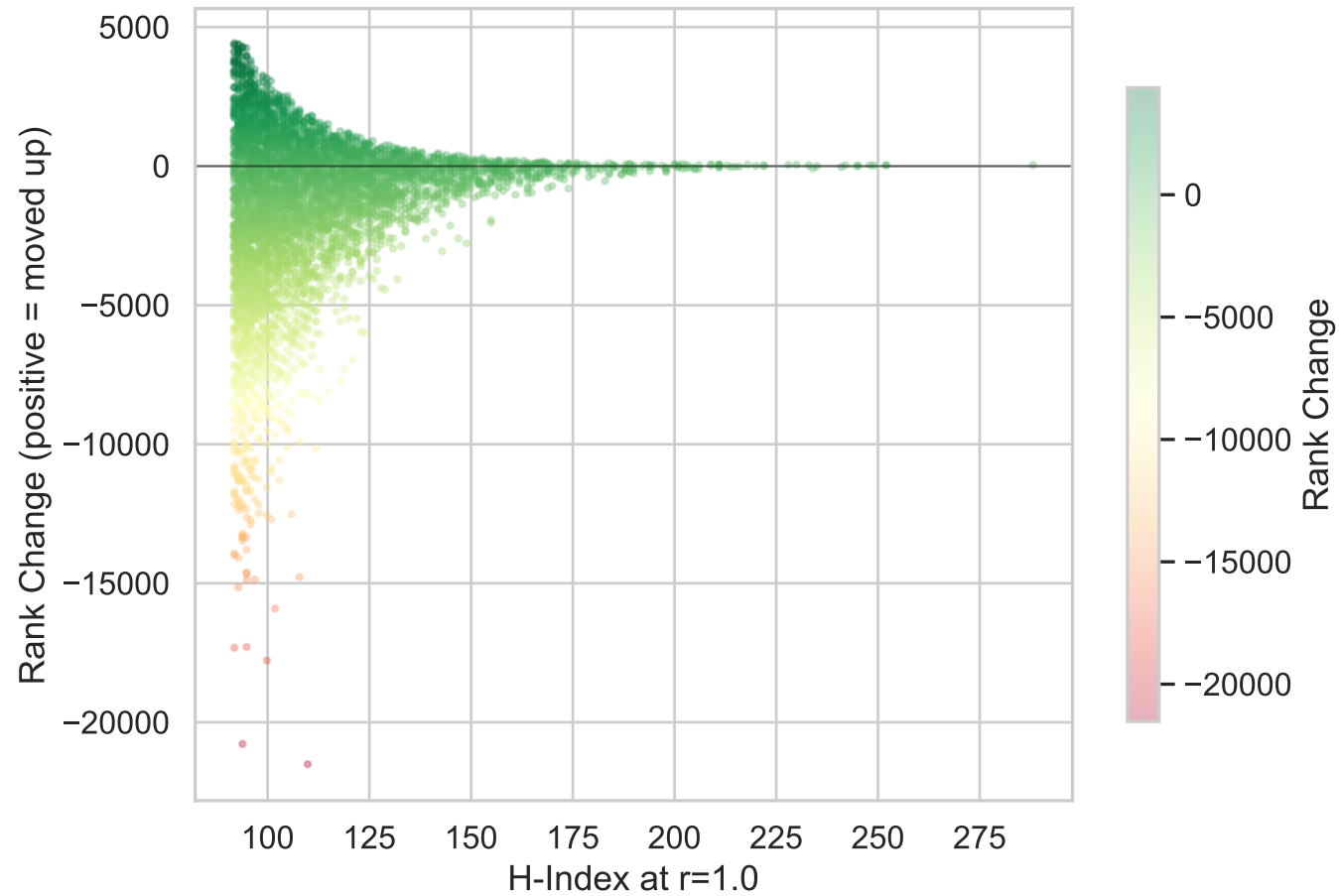
Rank Displacement (Top-5000)
