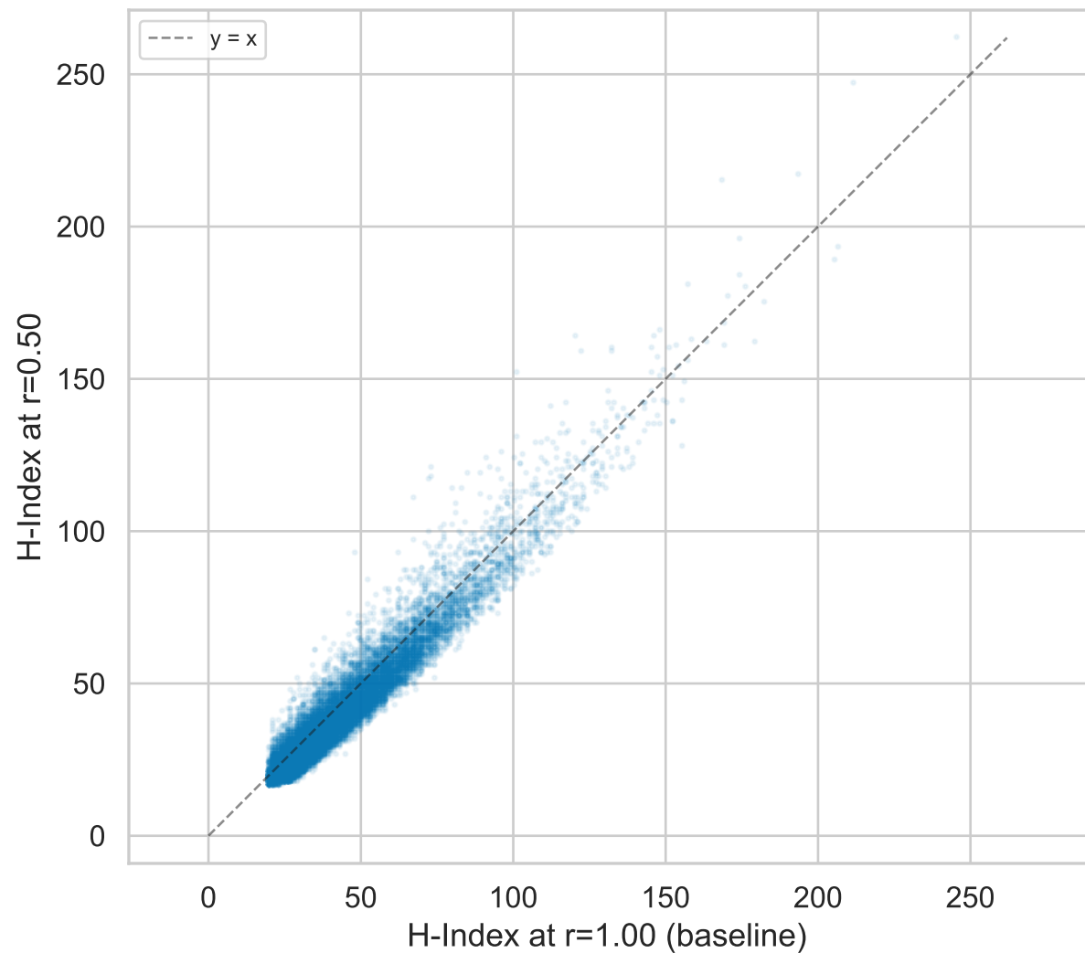
H-Index Scatter – r=1.0 \rightarrow r=0.50
