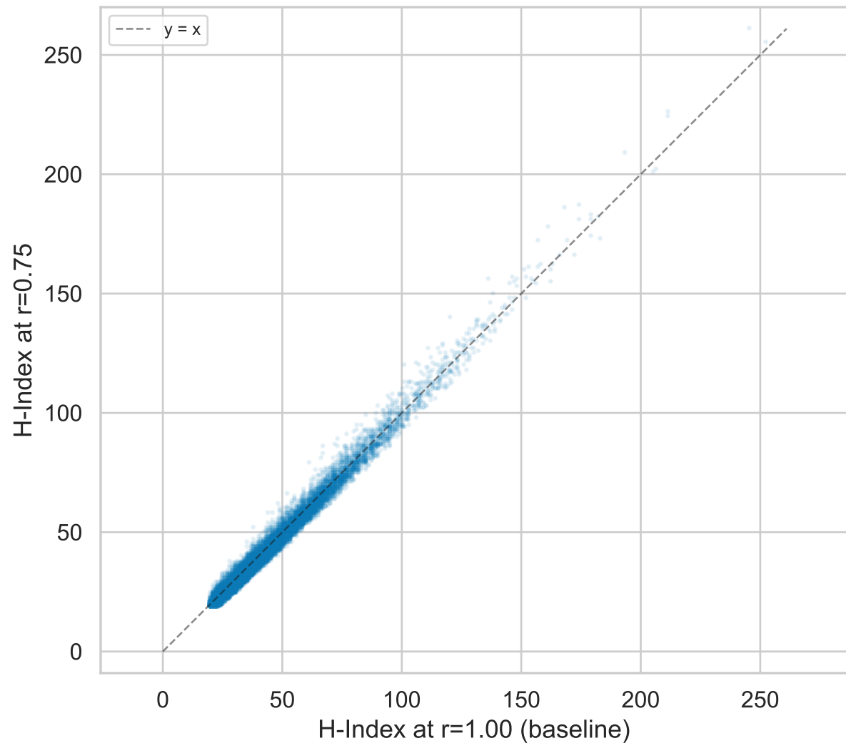
H-Index Scatter – r=1.0 \rightarrow r=0.75
