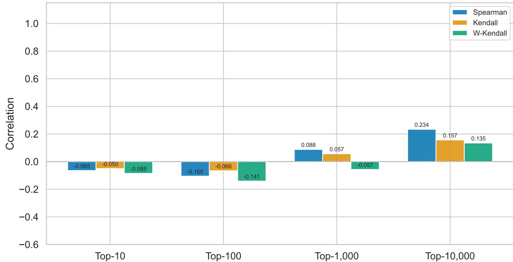
Rank Correlation vs Baseline - katz
