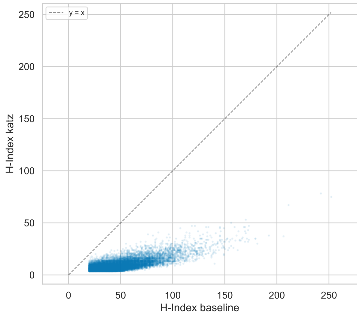
H-Index Scatter - baseline -> katz
