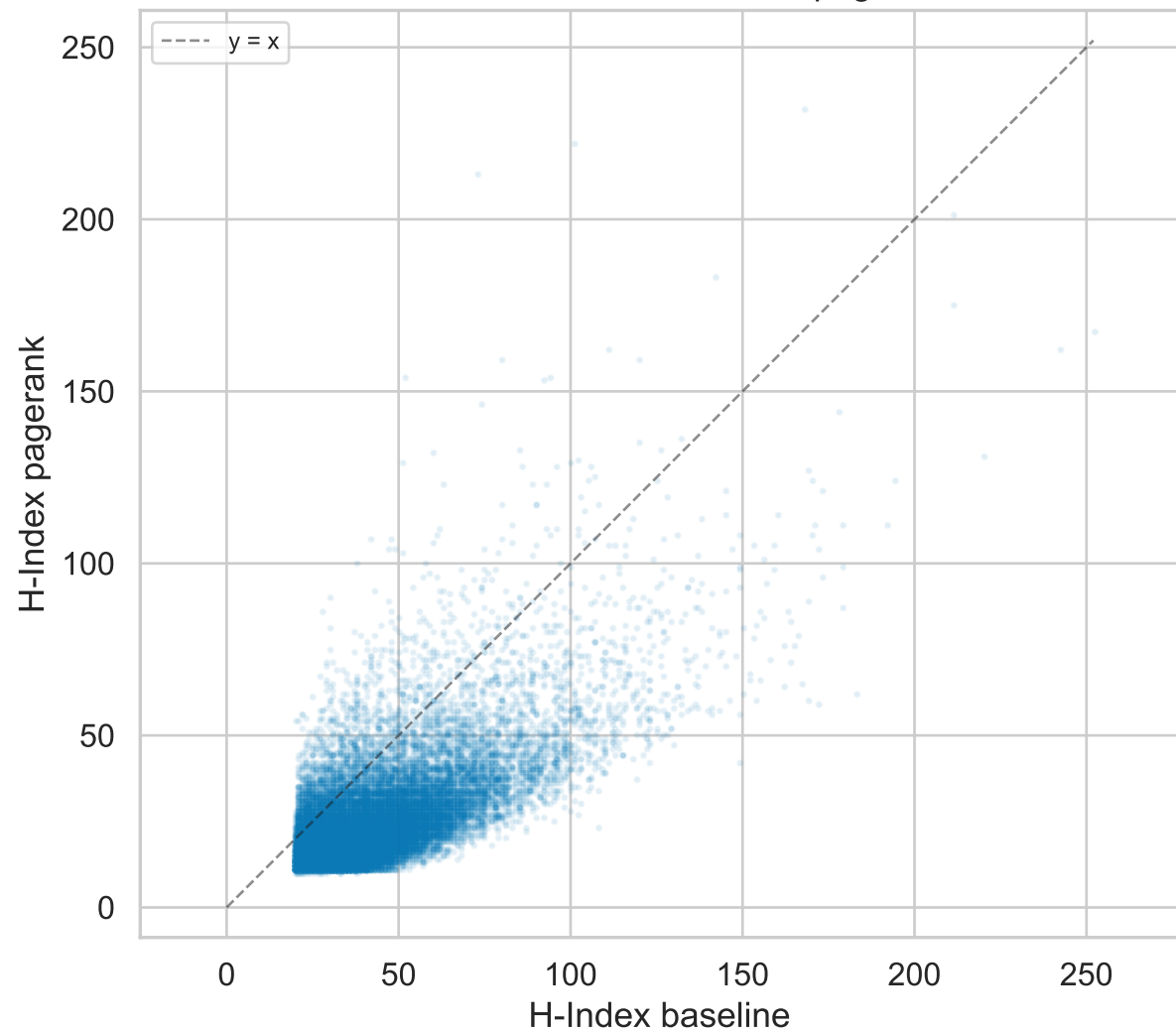
H-Index Scatter - baseline -> pagerank
