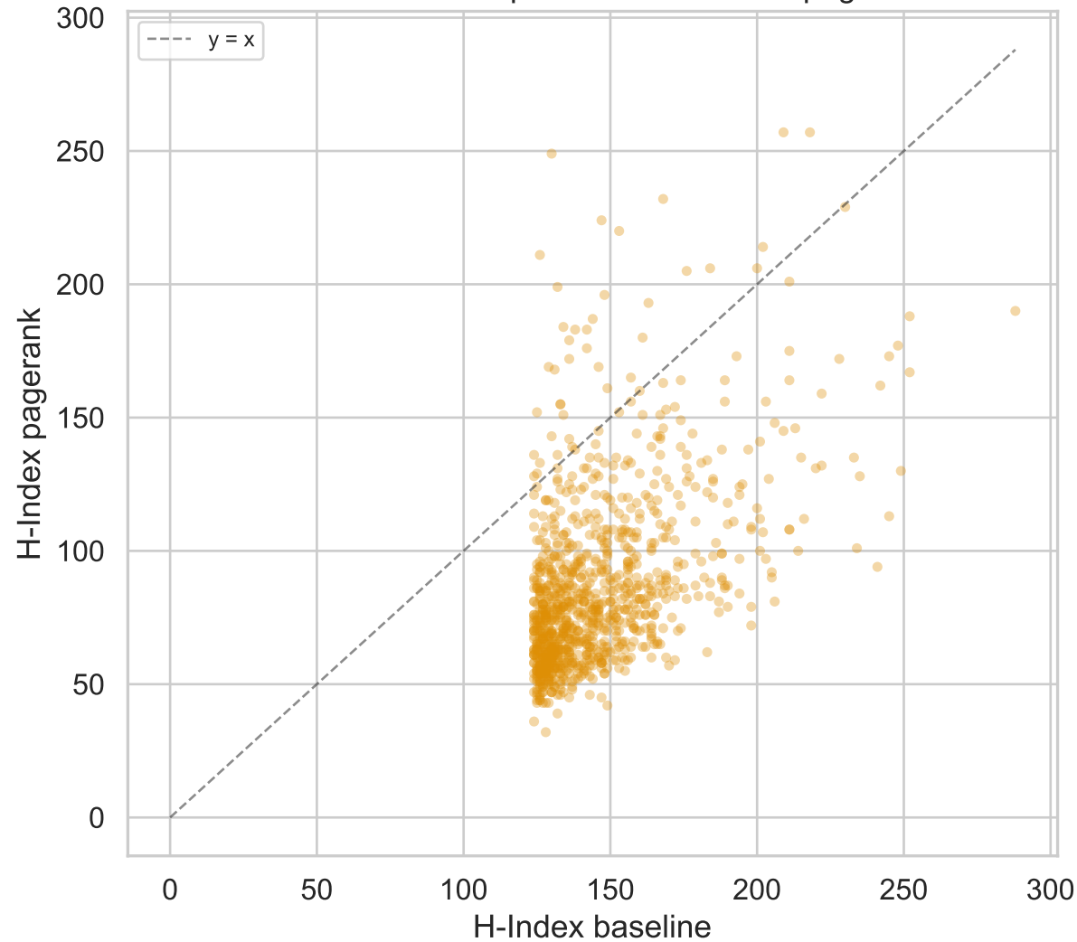
H-Index Scatter Top-1000 - baseline -> pagerank
